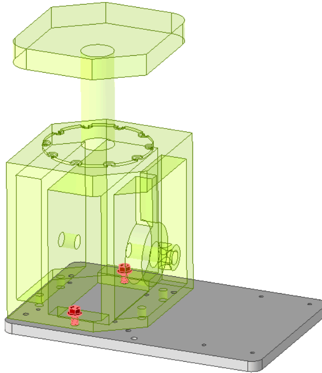
Figure 5.2c — Press aligned to base plate, M8 hardware installed loose
