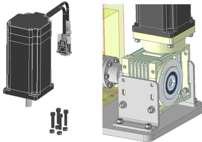
Figure 5.6b — NEMA 34 stepper motor installed into the gearbox
