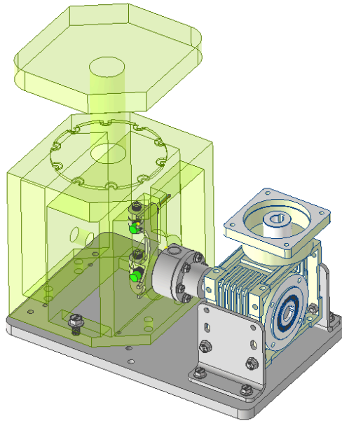
Figure 5.6a — Fully aligned assembly, ready to torque
