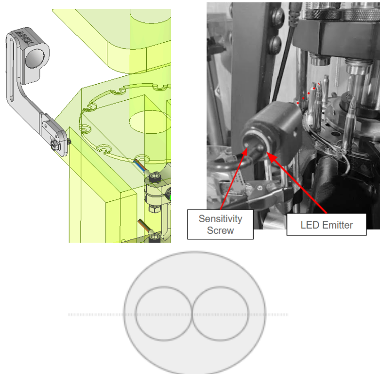
Figure 5.7a — Bullet sensor bracket mounting and alignment
