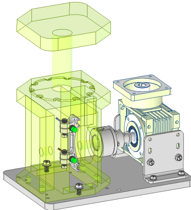
Figure 5.5b — Gearbox mounted to the L-brackets and base plate
