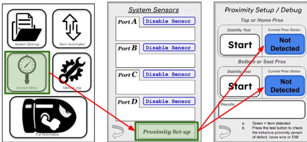
[ Figure 7.1a — Sensor page showing proximity sensor verification ]
