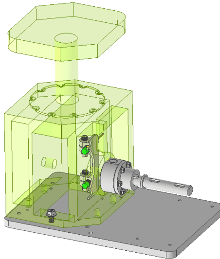
Figure 5.4b — Collar and shaft installation
