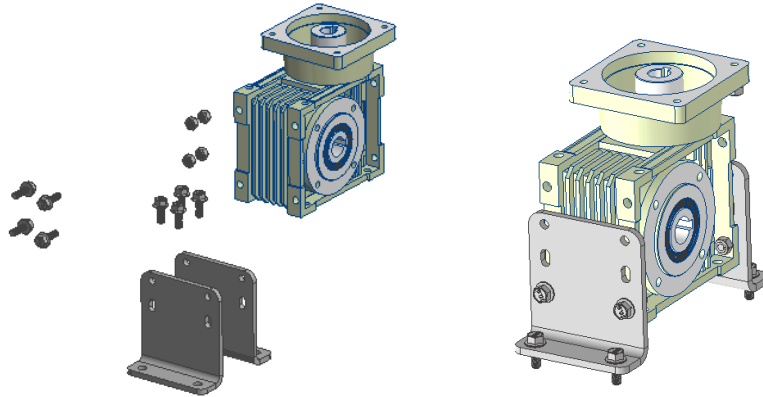
Figure 5.5a — L-bracket alignment and M6 × 20 flange bolt positions
