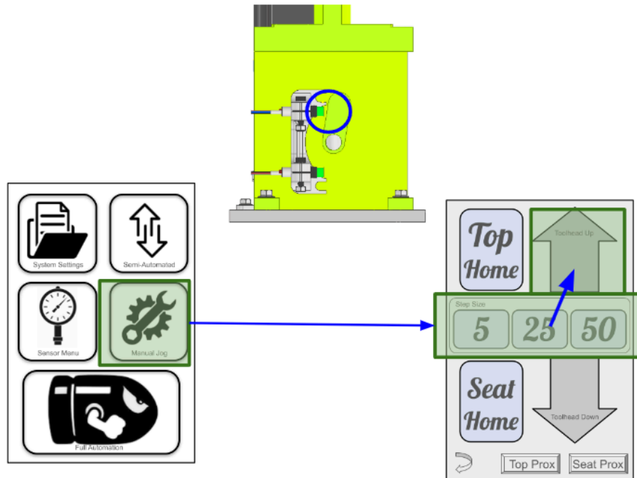
[ Figure 7.2a — Manual Jog screen and top proximity sensor position ]
