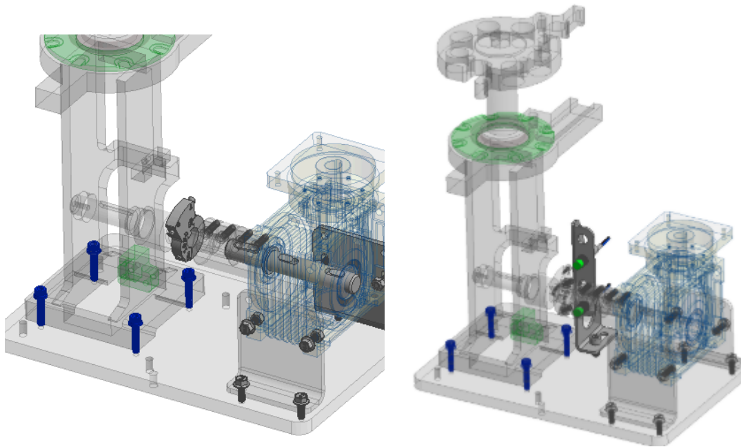
Figure 5.8b — Flag installed on keyed shaft, T and B markings facing outward
