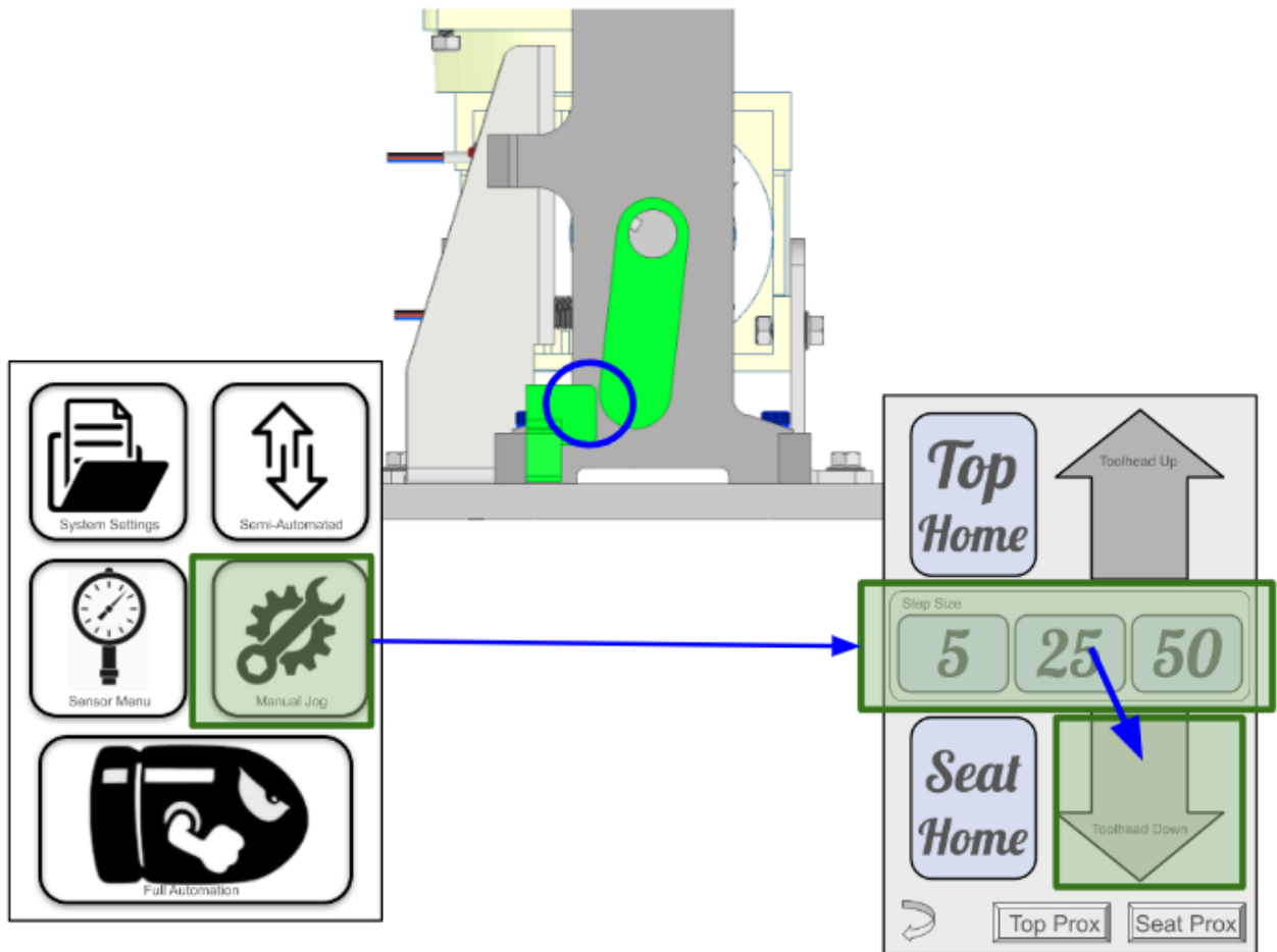
[ Figure 7.3a — Setting the bottom proximity sensor and measuring the gap ]
