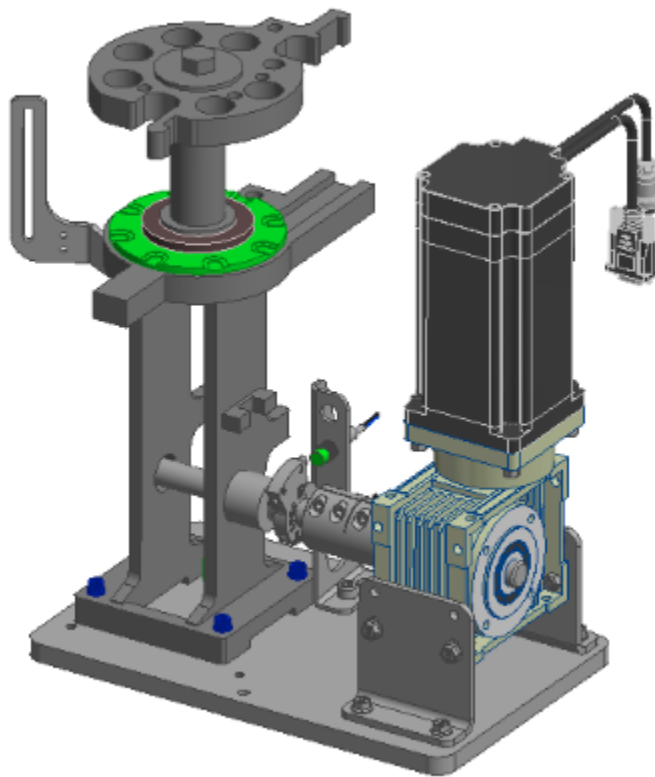
Figure 5.10a — Completed assembly
