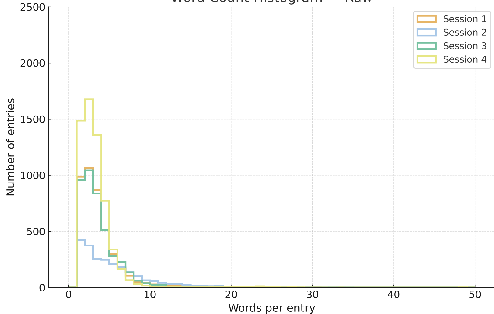
Word Count Histogram — Raw
