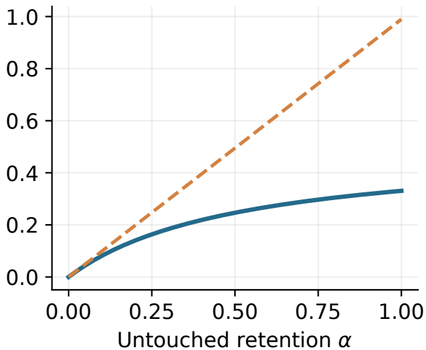
B: selection in U
