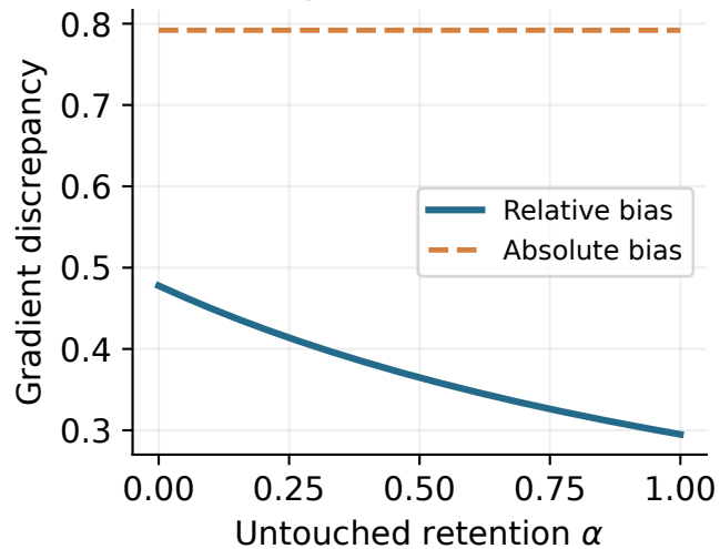
A: aligned, unbiased U
