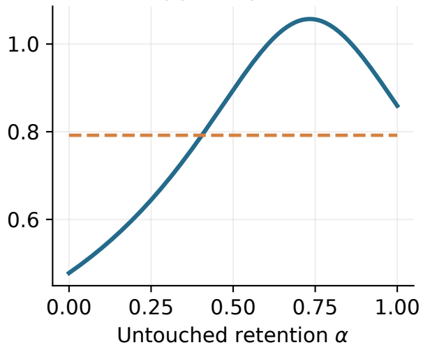
C: opposing means
