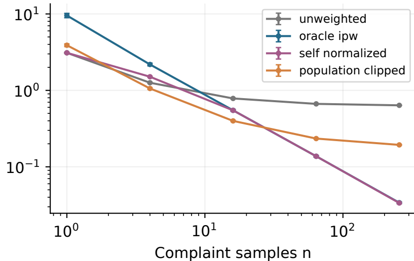
Retention \alpha = 1
