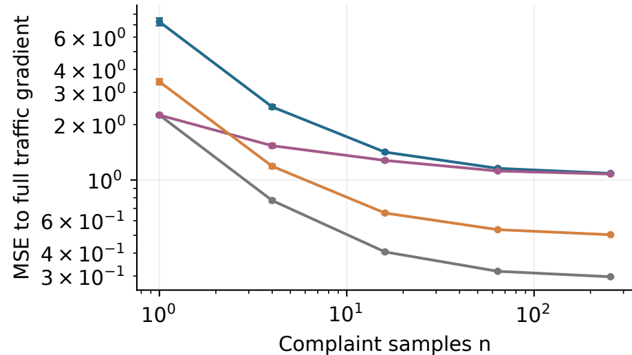
Retention \alpha = 0
