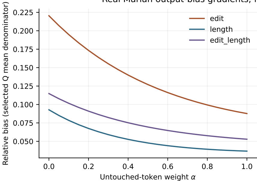
Real Marian output-bias gradients; human post-edits; synthetic selection
