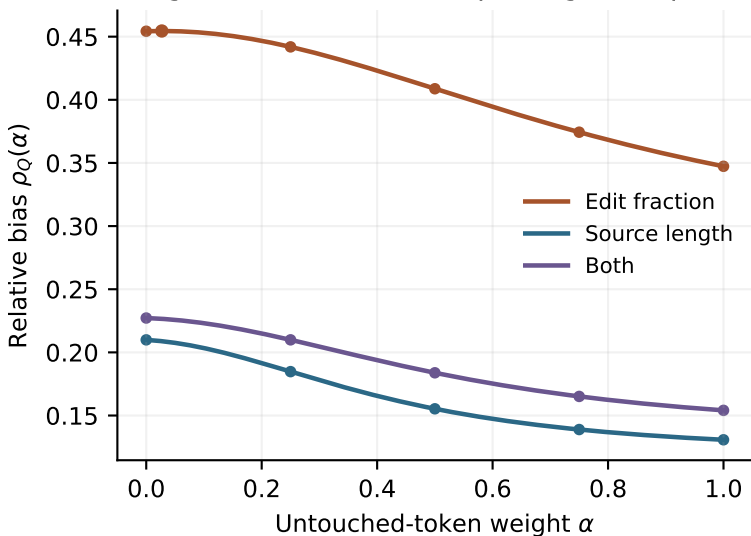
English-German (256 reporting examples)
