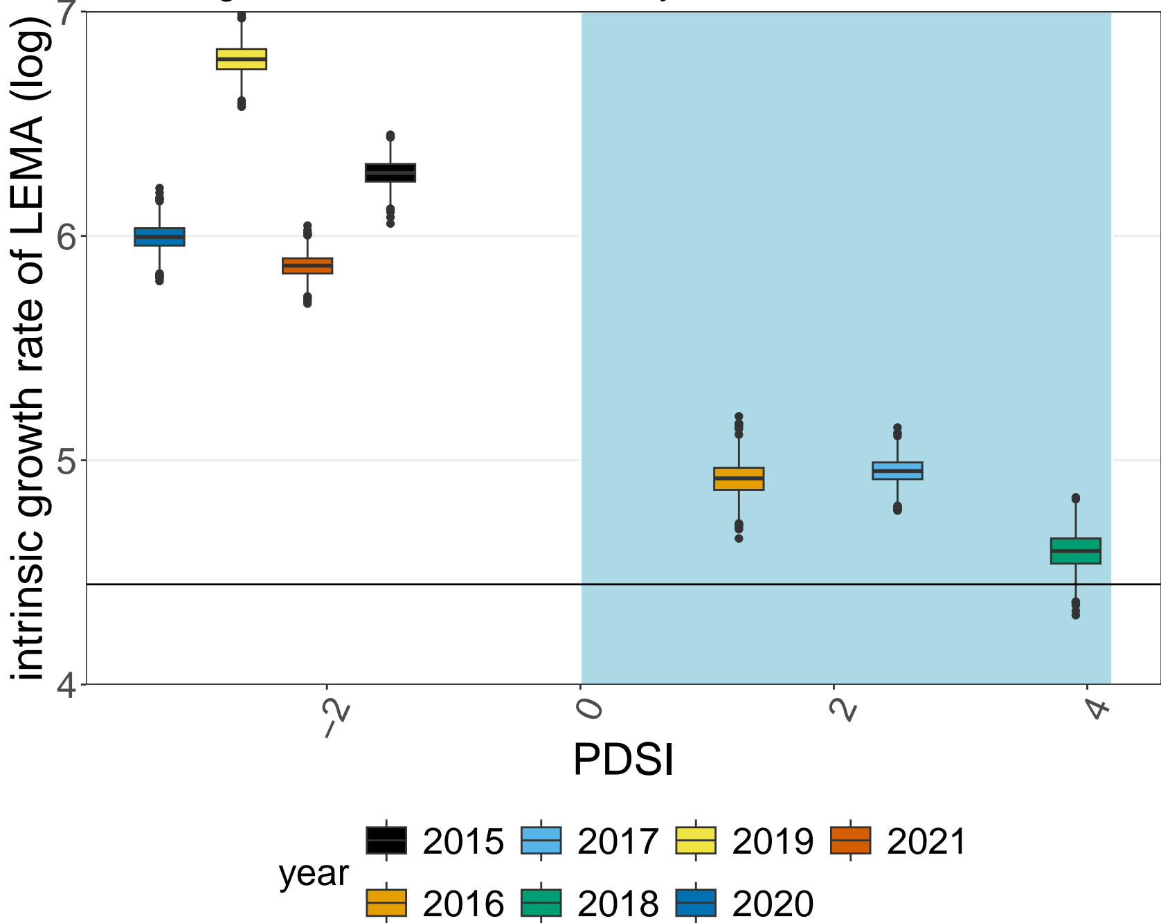
Intrinsic growth rate of LEMA across years, as their mean PDSI
