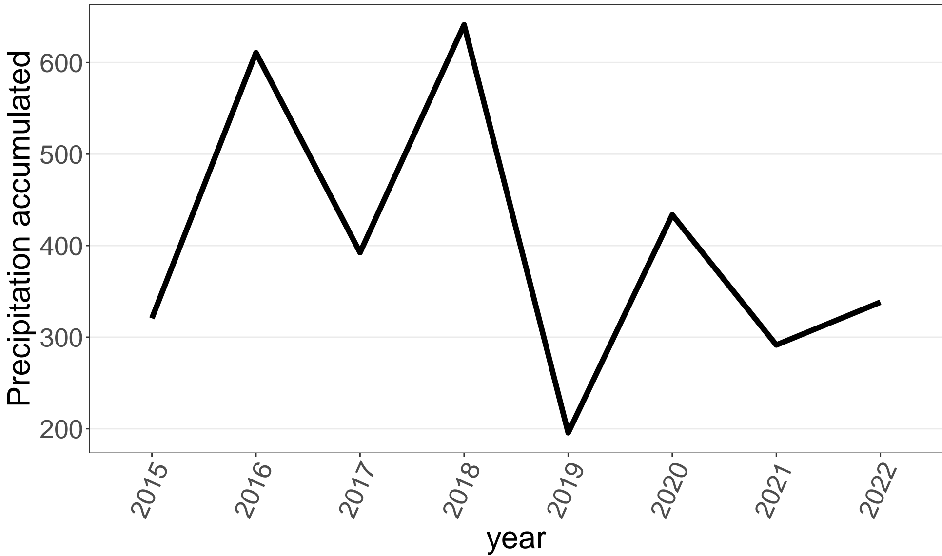
Precipitation over years, summed for each season
