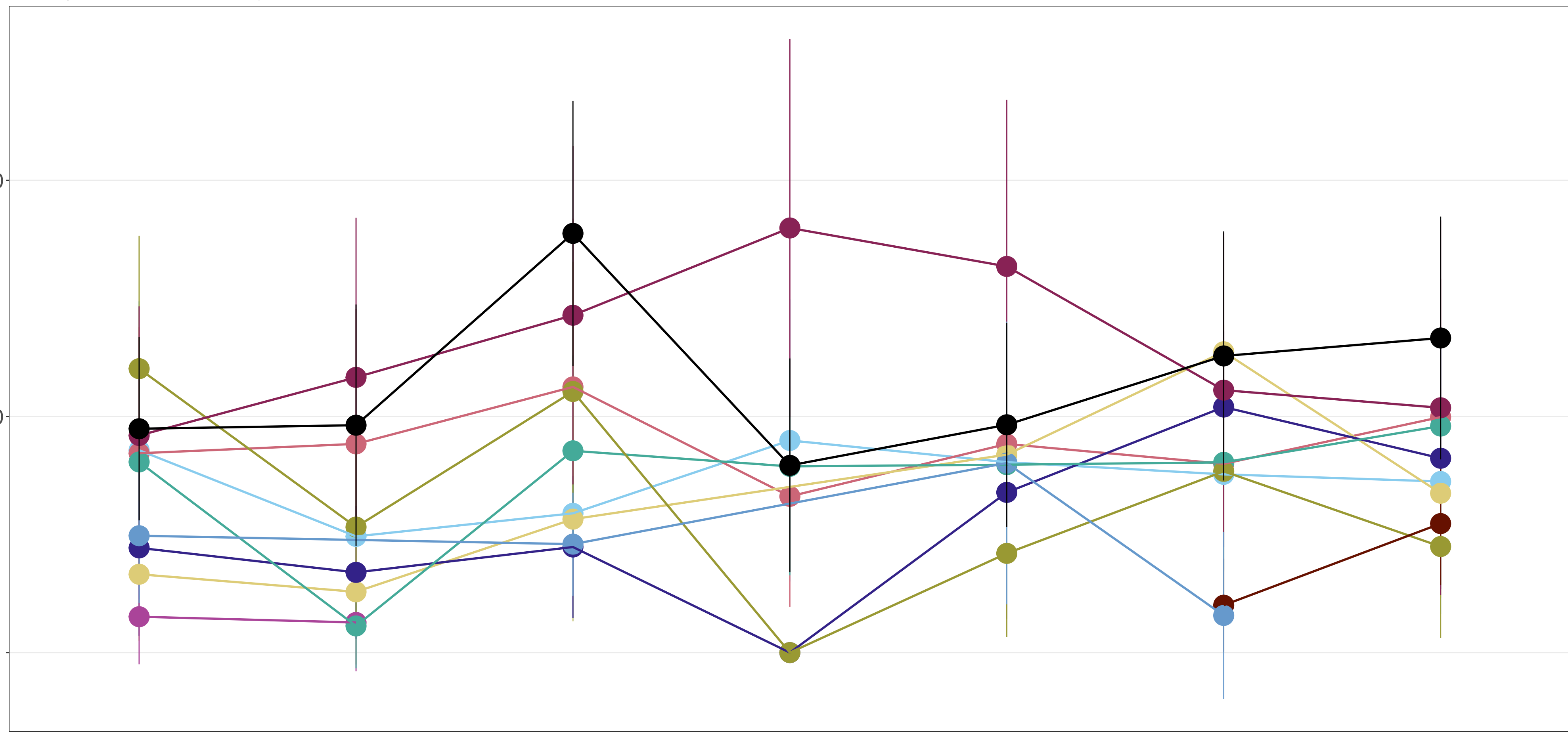
Density over time of annual plants in Caracoles
