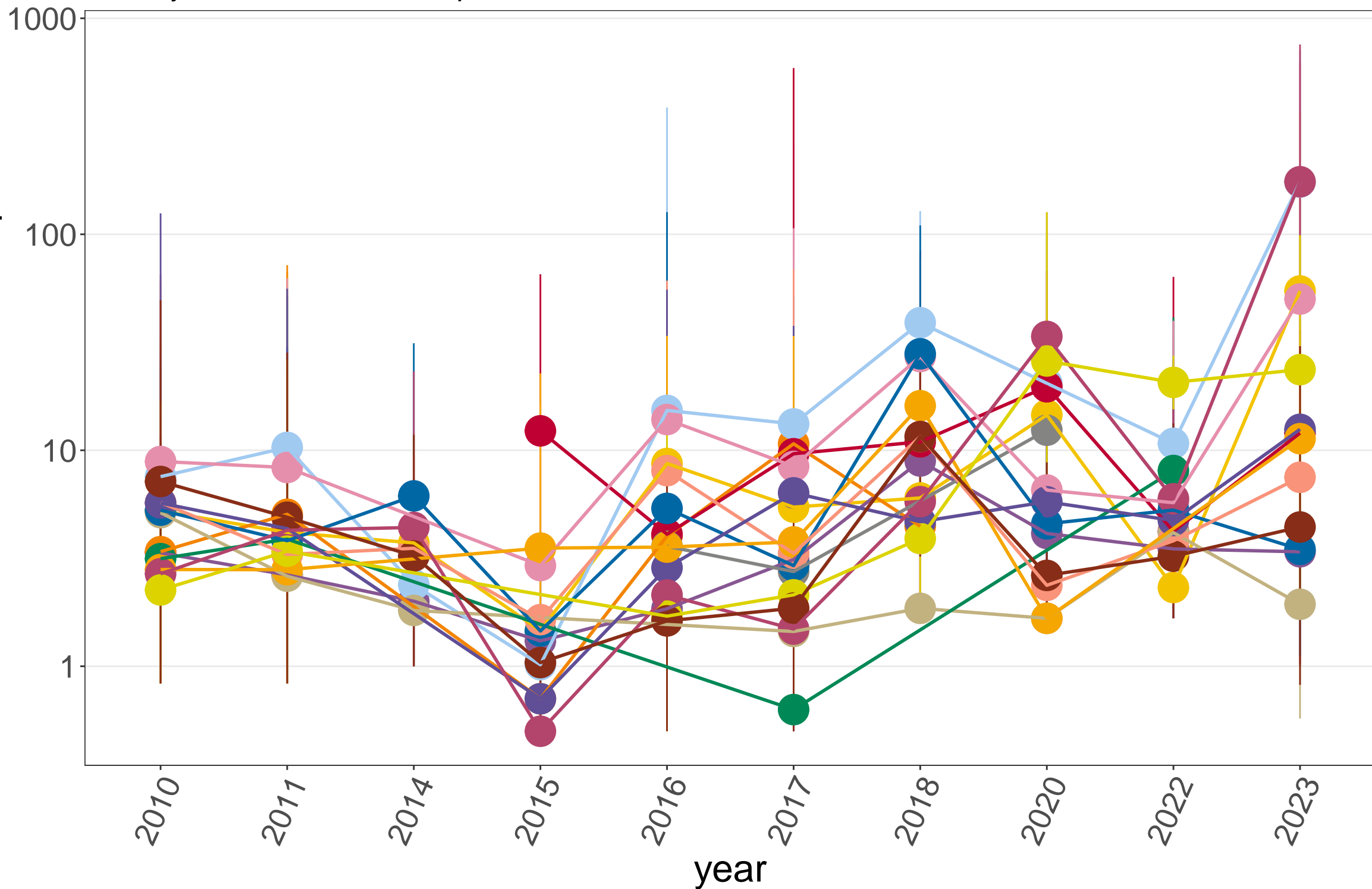
Density over time of annual plants in aus
