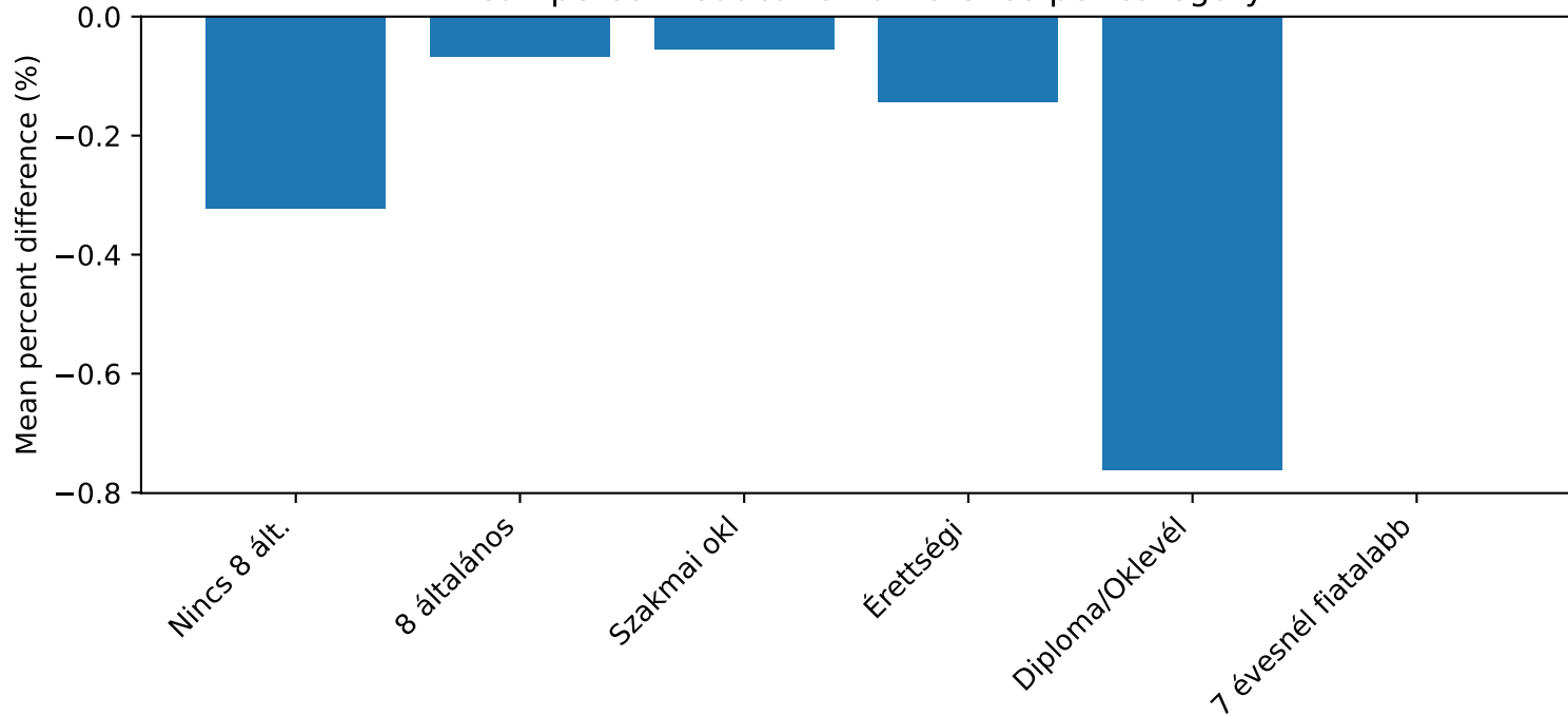
Mean percent education difference per category
