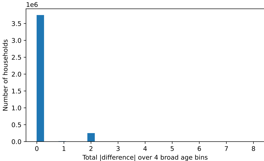
Total absolute age-bin difference per household (private)
