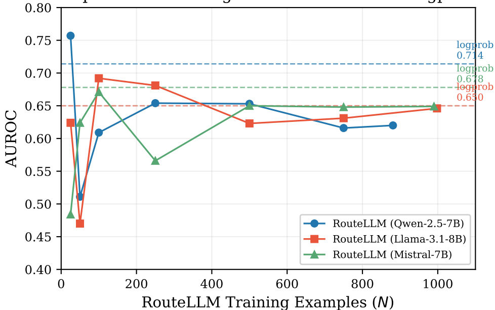
Supervised Learning Curve vs. Zero-Shot Logprob
