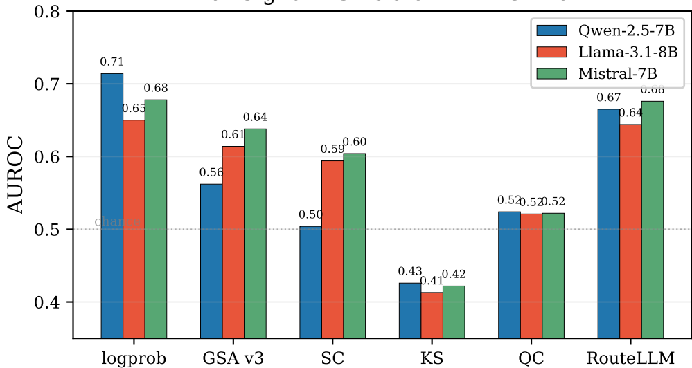
Per-Signal AUROC on MMLU-Pro
