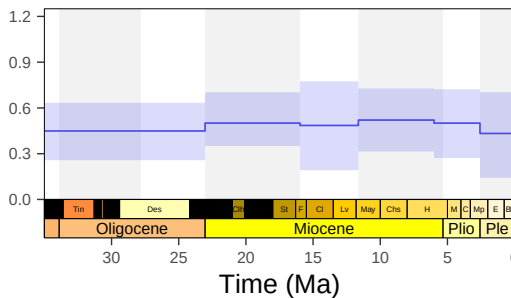
Speciation rate (r.10)
