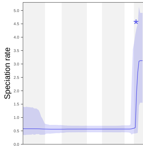
rjMCMC
