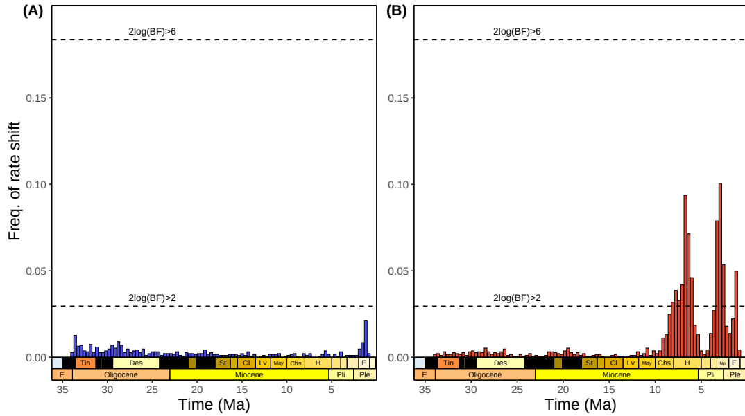
Figure S 5. Frequency of speciation (A) and extinction (B) rate shifts as estimated by the analysis of our genus-level chinchilloid occurrence dataset with the rjMCMC model. Dashed horizontal lines indicate 2 * \log(\text{Bayes factor}) of 2 and 6, respectively suggesting significant and strongly-supported rate shifts.
