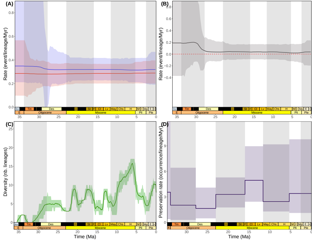
Figure S 6. Speciation and extinction (A), net diversification (= origination - extinction) (B) rates, diversity (C) and preservation rate (D) through time as estimated by the analysis of our species-level occurrence dataset with the rjMCMC model after removing singletons.
