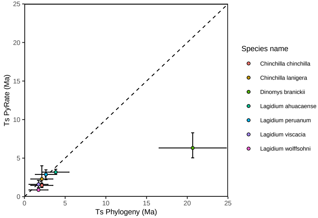
Figure S 15. Correspondance between divergence times leading to extant species estimated from our phylogeny ('Ts Phylo') and the times of species origination de novo estimated ('Ts PyRate') after implementing our sampling scheme for extant species absent from the fossil record ( Main text , Fig. 1). Dots show mean estimates and error bars the associated 95% HPD. Dashed line shows the line with equation y = x .
