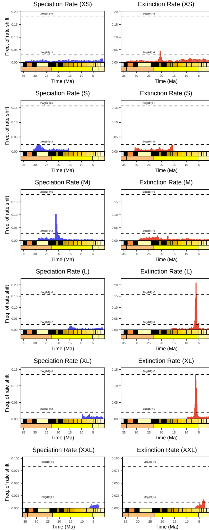
Figure S 10. Frequency of speciation and extinction rate shifts per body size class as estimated by the analysis of our species-level chinchilloid occurrence dataset with the rjMCMC model. Dashed horizontal lines indicate 2 \cdot \log(\text{Bayes factor}) of 2 and 6, respectively suggesting significant and strongly-supported rate shifts.
