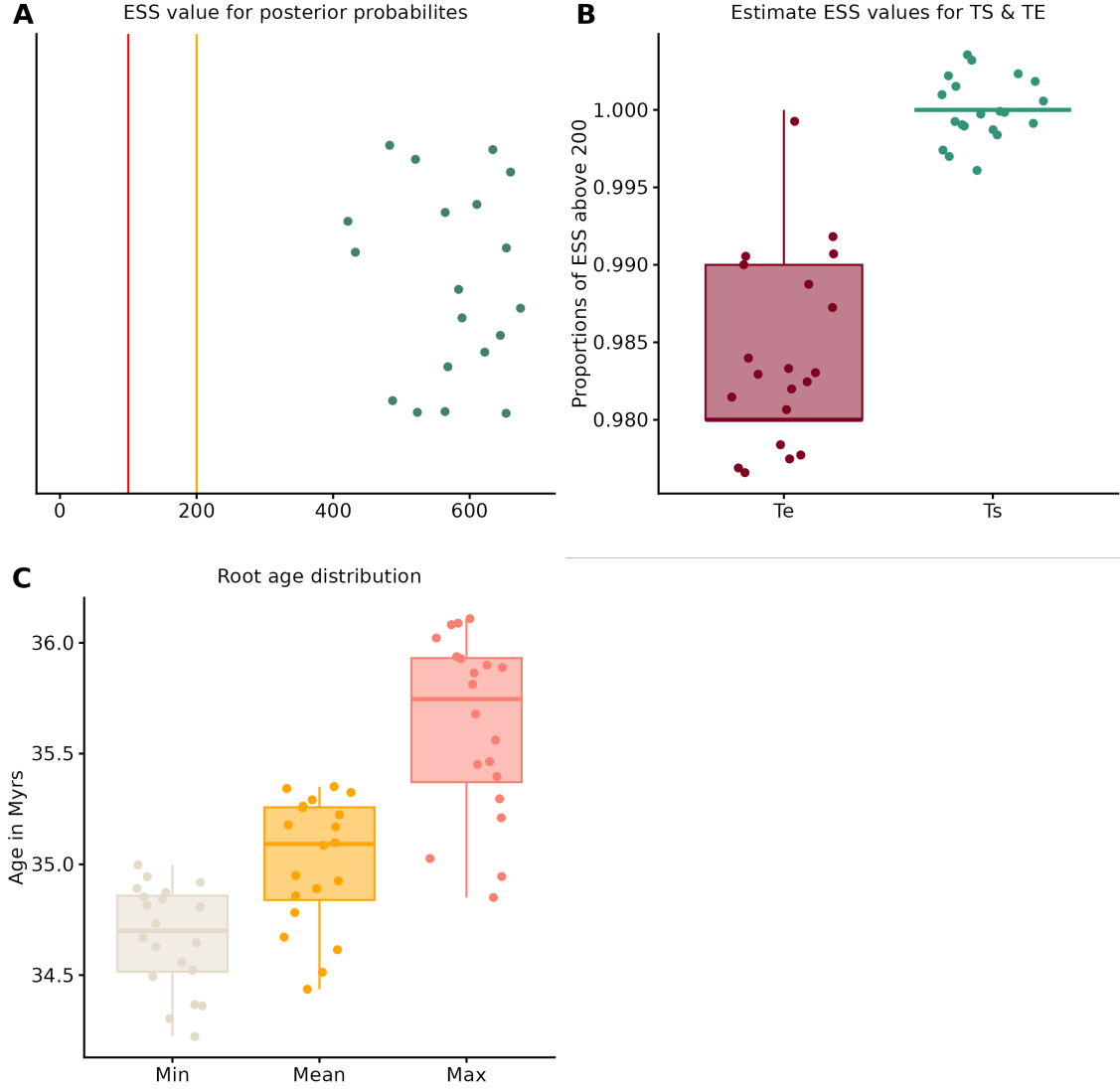
Figure S 3. Convergence of the PyRate runs for the analysis of the species-level temporal occurrence database. The plot (A) the ESS of the model posterior probability for all the 20 replicates we ran. ESS greater than 200 (first-scale indicator of a run that converged, n = 20 in that case) are displayed in green. The proportion of origination and extinction times (resp. T_S and T_E ) that converged (i.e., with ESS > 200 ) are shown in (B), for each of our 20 replicates. The plot (C) shows the posterior estimates of the mean root age of our group, together with their lower and upper boundaries of the 95% HPD interval, across the 20 replicates.
