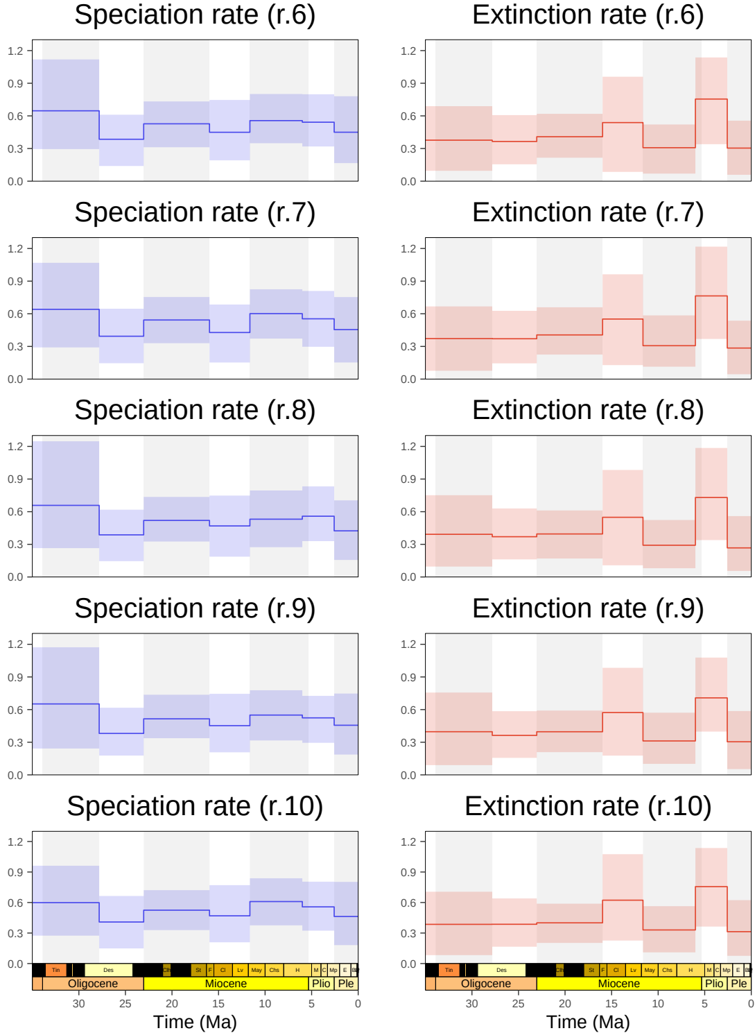
Figure S 12. Marginal chinchilloid speciation (blue) and extinction (red) rates through time as estimated by our BDNN analyses of the datasets with random trait ( i.e. , body mass and/or hypsodonty index) imputation for taxa with missing trait reconstruction ( n = 11 ). Caribbean taxa were excluded. Full lines show median rate estimates and ribbons their associated 95% Highest Posterior Density (HPD) interval, assessed across the 10 independent BDNN runs randomising fossil ages under a uniform law made for each trait imputation. This panel only depicts the rates through time from replicate 1 to 5.
