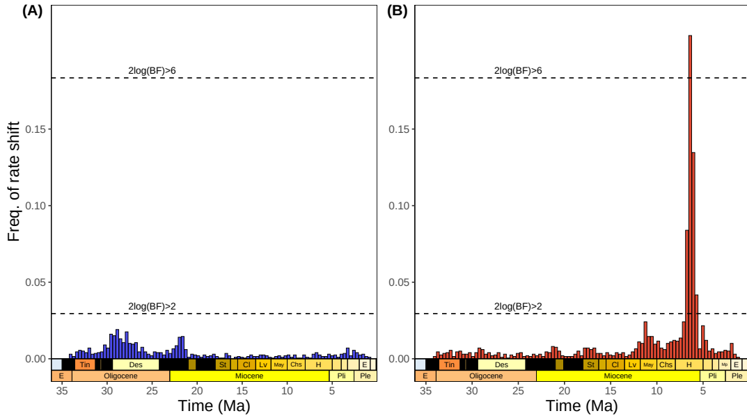
Figure S 2. Frequency of speciation (A) and extinction (B) rate shifts as estimated by the analysis of our species-level chinchilloid occurrence dataset with the rjMCMC model. Dashed horizontal lines indicate 2 * \log(\text{Bayes factor}) of 2 and 6, respectively suggesting significant and strongly-supported rate shifts.
