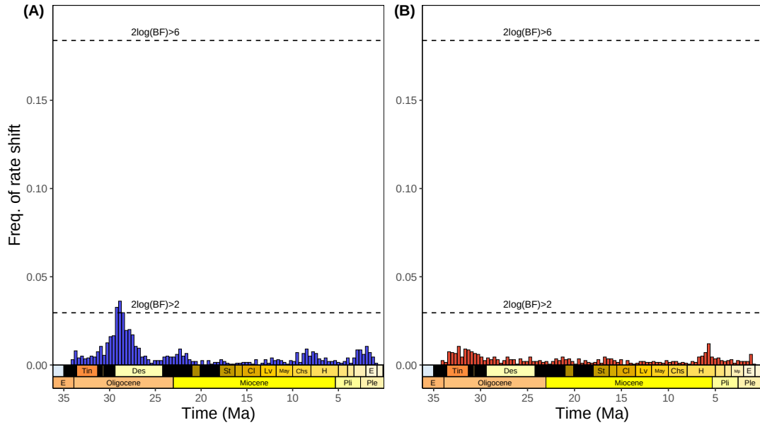
Figure S 7. Frequency of speciation (A) and extinction (B) rate shifts as estimated by the analysis of our species-level chinchilloid occurrence dataset with the rjMCMC model after removing singletons. Dashed horizontal lines indicate 2 * \log(\text{Bayes factor}) of 2 and 6, respectively suggesting significant and strongly-supported rate shifts.
