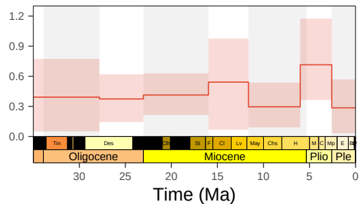
Extinction rate (r.10)
