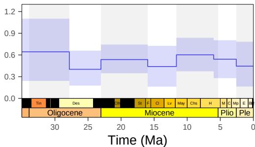
Speciation rate (r.10)
