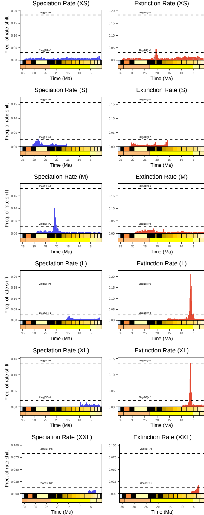
Figure S 9. Frequency of speciation and extinction rate shifts per body size class as estimated by the analysis of our species-level chinchilloid occurrence dataset with the rjMCMC model. Dashed horizontal lines indicate 2 \log(\text{Bayes factor}) of 2 and 6, respectively suggesting significant and strongly-supported rate shifts.
