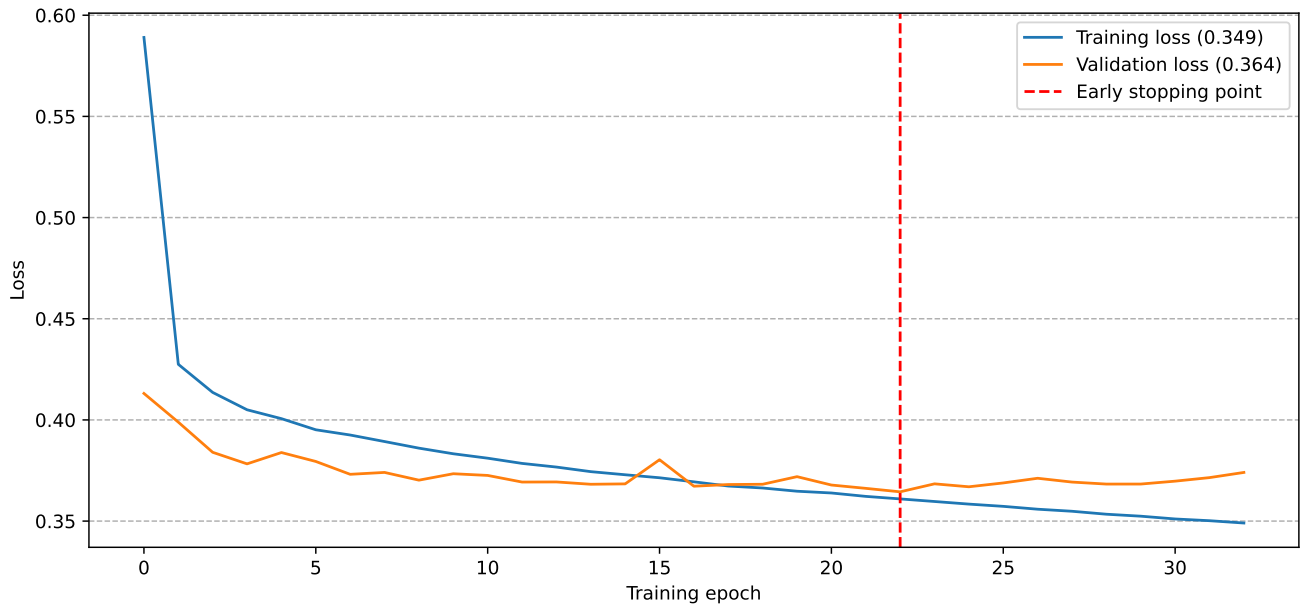
Figure S 13. Training and validation loss across training epochs for a DeepDive network comprising three LSTM units (128, 64 and 32 nodes) connected to two dense layers (64 and 32 nodes) before the output layer. The red vertical line indicates the “early stopping point”, i.e. , when the validation loss starts increasing, indicative of overfitting. It determines the optimal value of number of iterations, at which we derive the training and validation loss values depicted between parenthesis.
