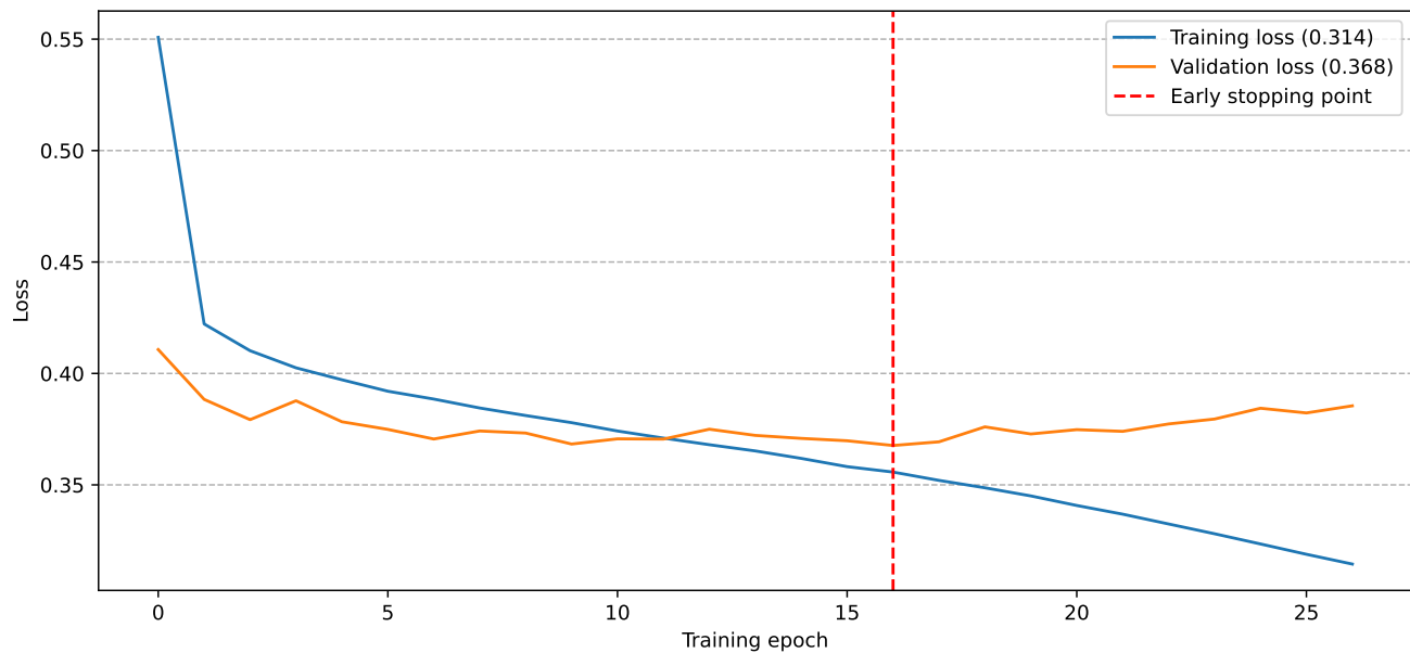
Figure S 12. Training and validation loss across training epochs for a DeepDive network comprising two LSTM units (64 and 32 nodes) connected to two dense layers (64 and 32 nodes) before the output layer. The red vertical line indicates the “early stopping point”, i.e. , when the validation loss starts increasing, indicative of overfitting. It determines the optimal value of number of iterations, at which we derive the training and validation loss values depicted between parenthesis.
