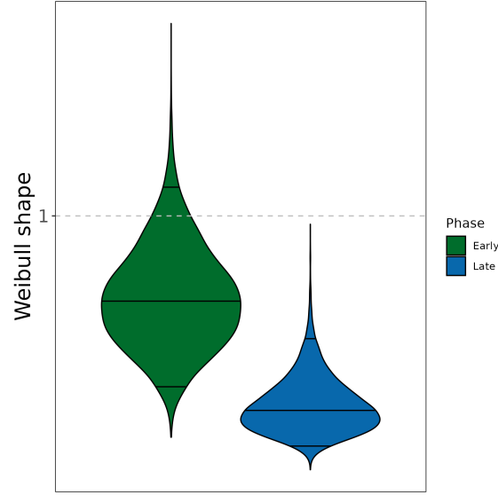
Figure S 4. Posterior estimate of the shape parameter of the Weibull distribution for the ADE analyses of the ‘Early’ (> 6 Ma) and ‘Late’ (< 6 Ma) occurrence datasets, each with constant extinction rate (?@fig-FreqRateShift). 2.5%, 50% and 97.5% quantiles are indicated in the distribution of each parameter by black horizontal lines, respectively from bottom to top.
