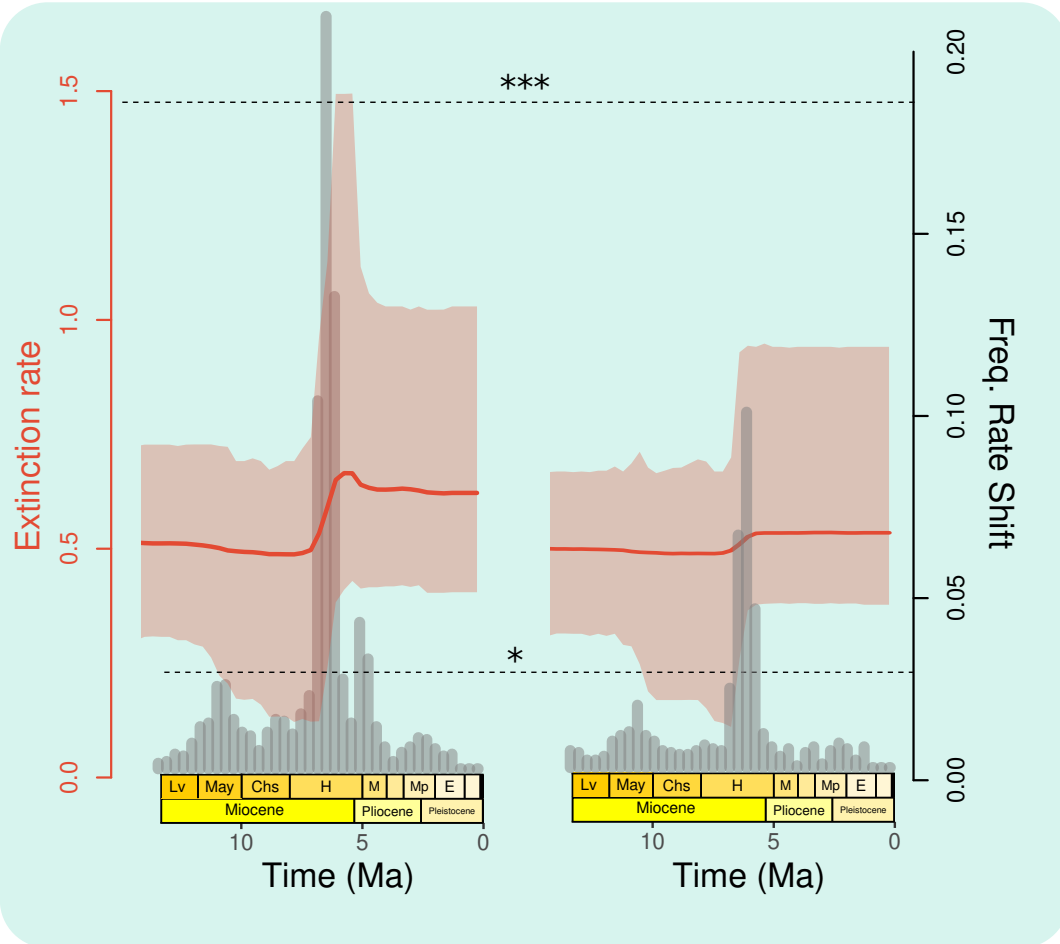
Figure S 3. Impact of incorporating the taxonomic revision of (?) about the dinomyid fauna of the Ituzaingó formation (Entre Ríos province, Argentina) on the estimation of the temporal dynamics of chinchilloid extinction rate. (A) Lifespans of species making up the fauna before (left) and after (right) the taxonomic revision. Removed taxa were coloured in red. (B) Chinchilloid extinction rates estimated from our temporal occurrence database with non-revised (left) and revised (right) dinomyids from the Ituzaingó formation. The histogram in background shows the frequency of rate shift estimated by the rjMCMC model, that is, for a given time frame (by default set to 1My), how likely it is to consider that the reconstructed extinction rate experienced a shift. The dashed lines labelled (*) and (***) respectively indicate significant and strongly supported rate shift.
