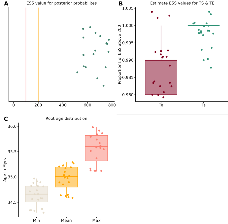
Figure S 2. Convergence of the PyRate runs for the analysis of the species-level temporal occurrence database. The plot (A) the ESS of the model posterior probability for all the 20 replicates we ran. ESS greater than 200 (first-scale indicator of a run that converged, n = 20 in that case) are displayed in green. The proportion of origination and extinction times (resp. T_S and T_E ) that converged (i.e., with ESS > 200 ) are shown in (B), for each of our 20 replicates. The plot (C) shows the posterior estimates of the mean root age of our group, together with their lower and upper boundaries of the 95% HPD interval, across the 20 replicates.
