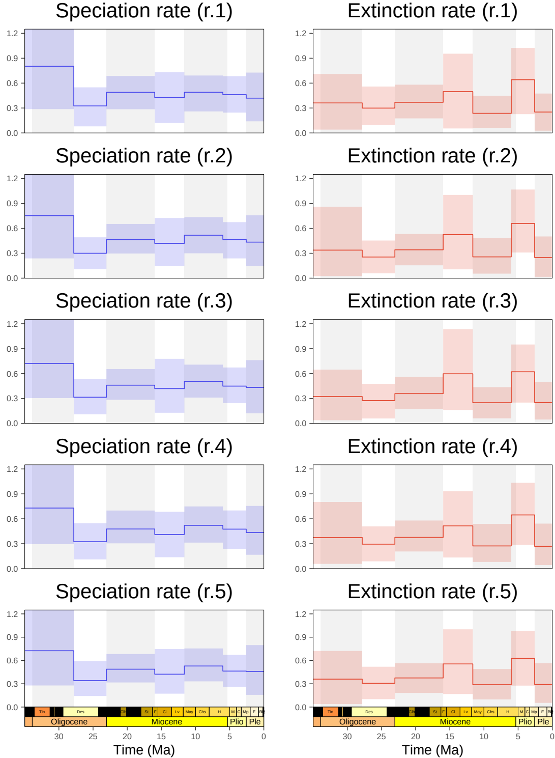
Figure S 7. Marginal chinchilloid speciation (blue) and extinction (red) rates through time as estimated by our BDNN analyses of the datasets with random trait ( i.e. , body mass and/or hypsodonty index) imputation for taxa with missing trait reconstruction ( n = 11 ). Caribbean taxa were excluded. Full lines show median rate estimates and ribbons their associated 95% Highest Posterior Density (HPD) interval, assessed across the 10 independent BDNN runs randomising fossil ages under a uniform law made for each trait imputation. This panel only depicts the rates through time from replicate 1 to 5.
