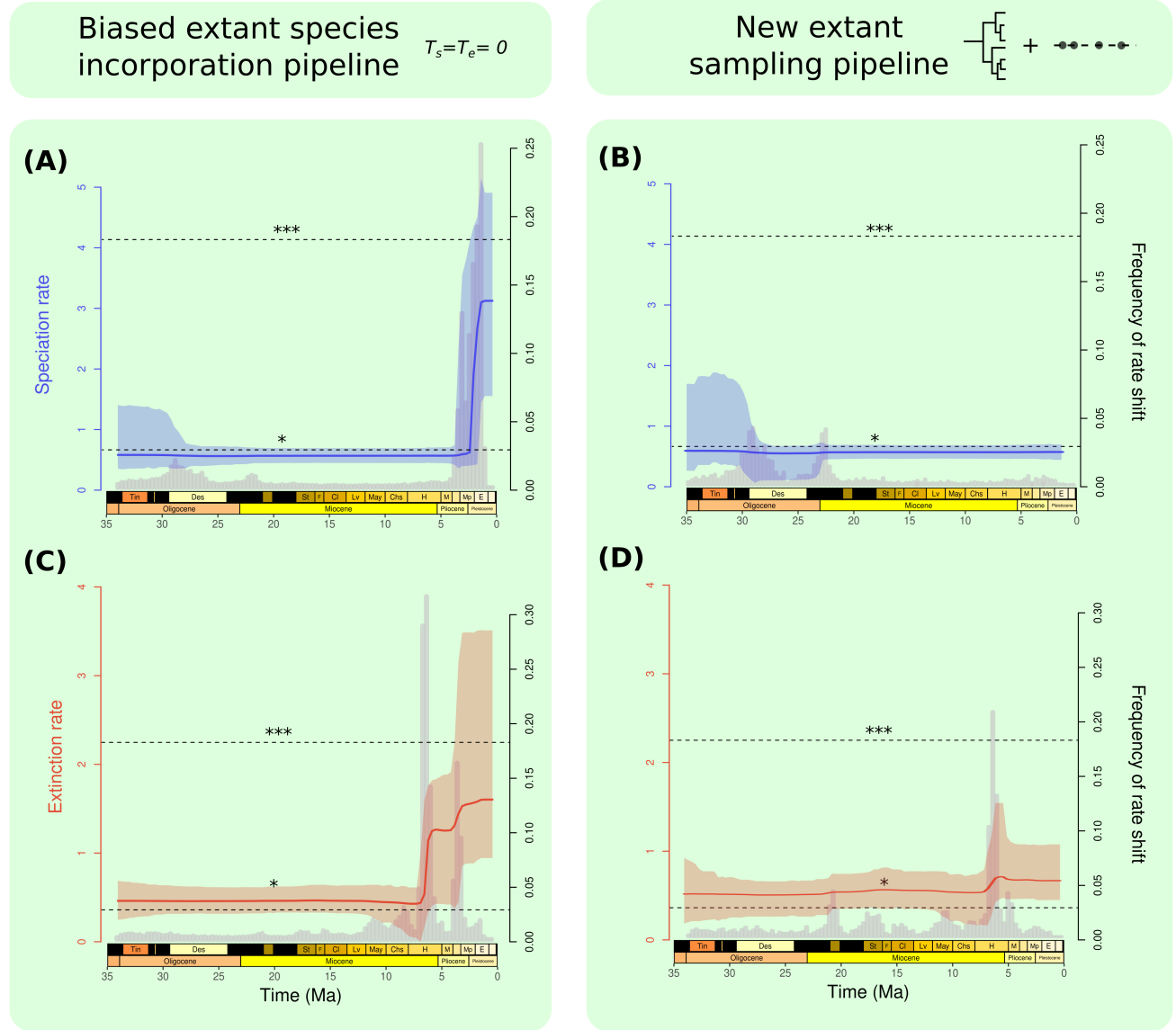
Figure S 2. Impact of the sampling scheme of extant species lacking fossil record on the estimation of speciation and extinction rates. Rates were estimated with PyRate using the rjMCMC algorithm, either from a dataset in which extant taxa were included by means of an occurrence with origination and extinction ages ( T_e and T_e ) set to 0 Ma ( A and C ) or with our newly-introduced pipeline relying on ages extracted from dated phylogenies ( B and D ). Full lines indicate median rate estimation (blue for speciation, red for extinction), and ribbons their associated 95% HPD interval. Grey histograms in the background depict the frequency of rate shift per 1-My time bins. The two horizontal lines labelled * and *** respectively indicate significant and strongly supported rate shift. Note that, in the two cases, these results were obtained prior to the incorporation of the taxonomic revision of the ‘Mesopotamian’ dinomyid fauna (Ituzaingó Fm.) made by Rasia (2026) (see Figure S12 for the subsequent effect of incorporating this revision on diversification rate estimation).
