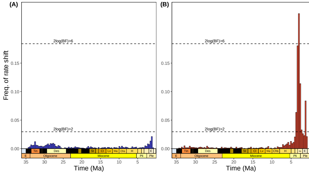
Figure S 10. Frequency of origination ( A ) and extinction ( B ) rates estimated by the rjMCMC analysis of our genus-level database.
