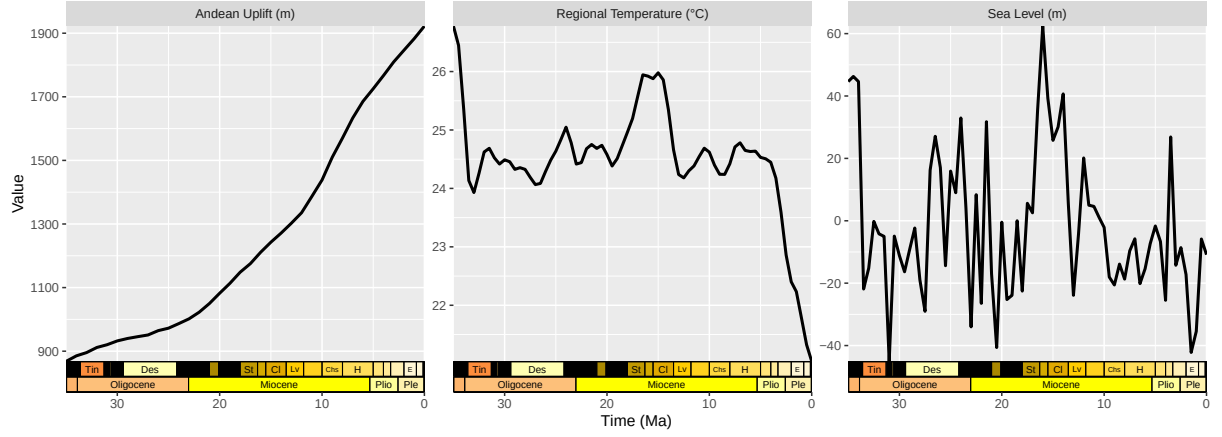
Figure S 22. Abiotic variables used in the environment-dependent diversification analyses carried out over this study. These have been temporally scaled to the same resolution (500ky-step). Andean uplift was from Boschman (2021), South American regional temperature was from Tardif et al. (2025) and sea-level changes were from Miller et al. (2020).
