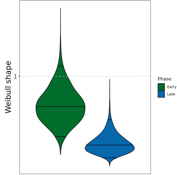
Figure S 12. Posterior estimate of the shape parameter of the Weibull distribution for the ADE analyses of the ‘Early’ (> 6 Ma) and ‘Late’ (< 6 Ma) occurrence datasets, each with constant extinction rate (Figure S5). 2.5%, 50% and 97.5% quantiles are indicated in the distribution of each parameter by black horizontal lines, respectively from bottom to top.
