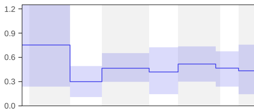
Speciation rate (r.3)
