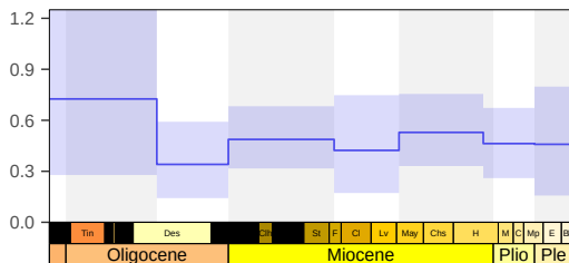
Speciation rate (r.5)
