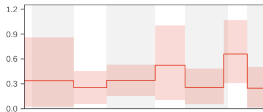
Extinction rate (r.3)
