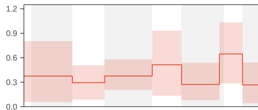
Extinction rate (r.5)
