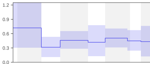
Speciation rate (r.4)
