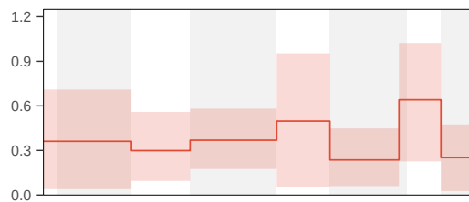
Extinction rate (r.2)
