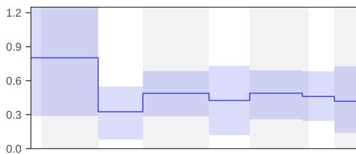
Speciation rate (r.2)
