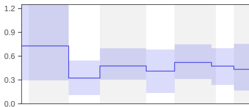
Speciation rate (r.5)
