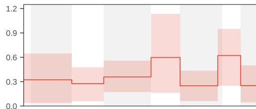
Extinction rate (r.4)
