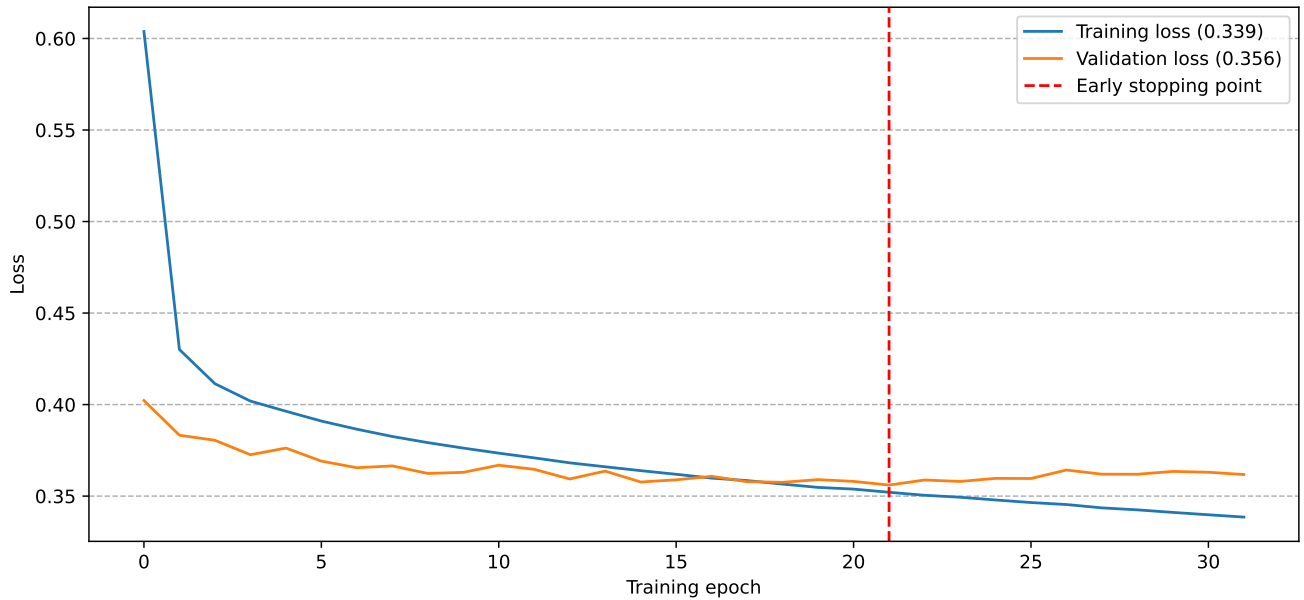
Figure S 8. Training and validation loss across training epochs for a DeepDive network comprising 2 LSTM units (64 and 32 nodes) connected to two dense layers (64 and 32 nodes) before the output layer. The red vertical line indicates the “early stopping point”, i.e. , when the validation loss starts increasing, indicative of overfitting. It determines the optimal value of number of iterations, at which we derive the training and validation loss values depicted between parenthesis.
