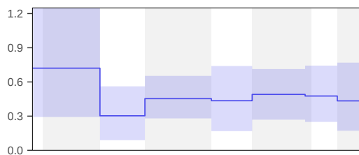
Speciation rate (r.7)
