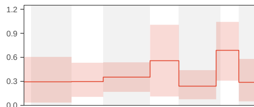
Extinction rate (r.8)
