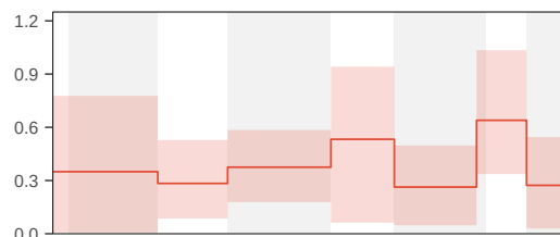
Extinction rate (r.9)
