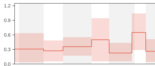
Extinction rate (r.7)
