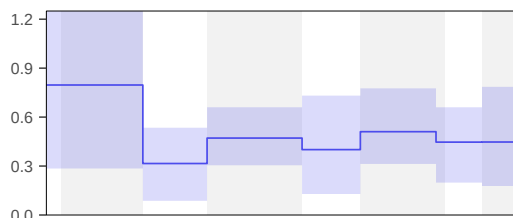
Speciation rate (r.9)
