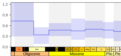
Speciation rate (r.10)
