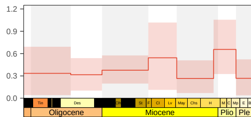
Extinction rate (r.10)
