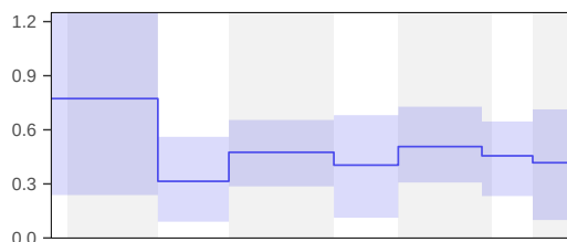
Speciation rate (r.10)
