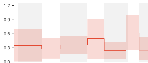
Extinction rate (r.10)
