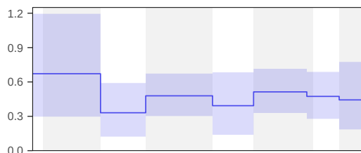
Speciation rate (r.8)
