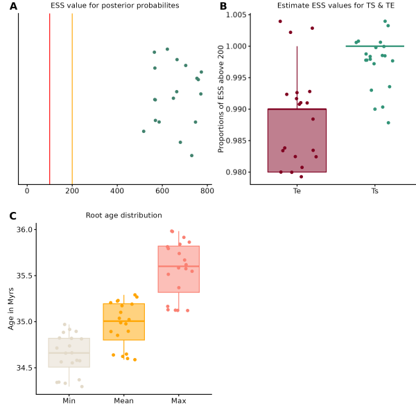
Figure S 4. Convergence of the PyRate runs for the analysis of the species-level temporal occurrence database. The plot (A) the ESS of the model posterior probability for all the 20 replicates we ran. ESS greater than 200 (first-scale indicator of a run that converged, n = 20 in that case) are displayed in green. The proportion of origination and extinction times (resp. T_S and T_E ) that converged (i.e., with ESS > 200 ) are shown in (B), for each of our 20 replicates. The plot (C) shows the posterior estimates of the mean root age of our group, together with their lower and upper boundaries of the 95% HPD interval, across the 20 replicates.
