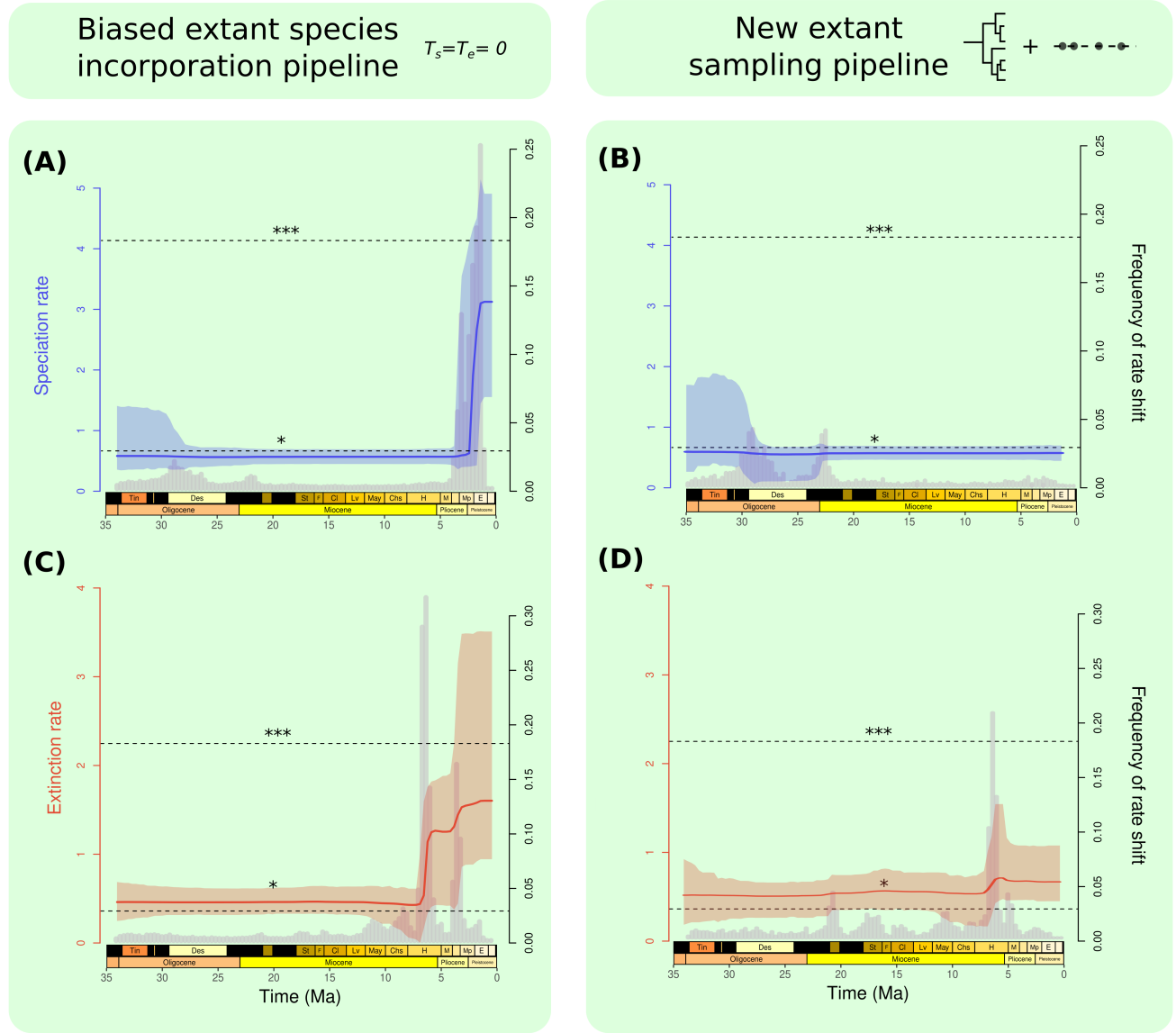
Figure S 1. Impact of the sampling scheme of extant species lacking fossil record on the estimation of speciation and extinction rates. Rates were estimated with PyRate using the rjMCMC algorithm, either from a dataset in which extant taxa were included by means of an occurrence with origination and extinction ages ( T_o and T_e ) set to 0 Ma (A and C) or with our newly-introduced pipeline relying on ages extracted from dated phylogenies (B and D). Full lines indicate median rate estimation (blue for speciation, red for extinction), and ribbons their associated 95% HPD interval. Grey histograms in the background depict the frequency of rate shift per 1-My time bins. The two horizontal lines labelled * and *** respectively indicate significant and strongly supported rate shift. Note that, in the two cases, the datasets used did not incorporate the taxonomic updates of the dinomyid fauna from the Ituzaingó Fm. made by Rasia (2026) (see Figure S11).
