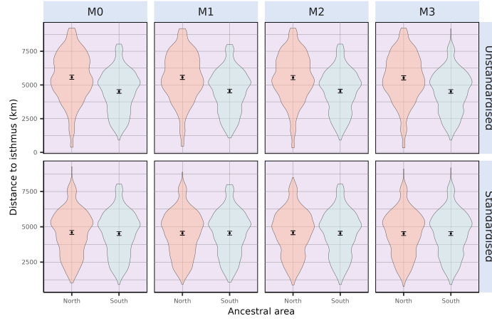
Figure S 1: Distribution of the distance to isthmus of the ancestral species of simulations either starting in North or South America, either resulting from our random equal-area sampling scheme ( top ) or from our spatial standardisation procedure ( bottom ) (see Section 1). Black dots in the middle of the distributions are mean estimates, and error bars represent their student-derived 95% confidence interval.
