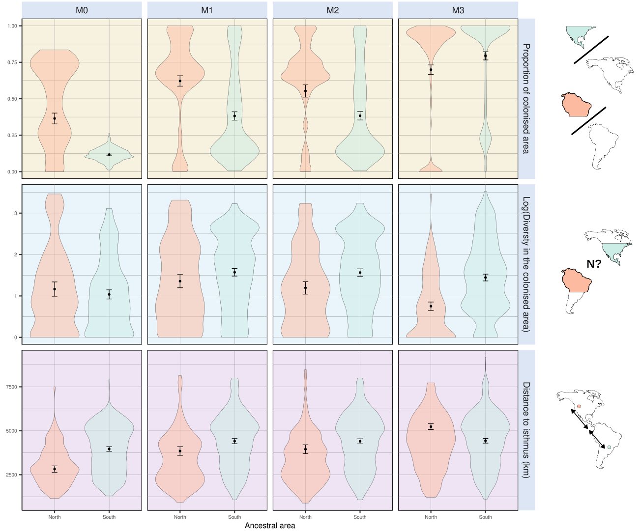
Figure S 3: A few metrics summarising climate-mediated interchange. Each individual plot shows the outcome of simulations starting in North (red) and South (cyan) America. ( top ) Proportion of foreign continent's colonised area. ( middle ) Diversity within the colonised area. ( bottom ) Distance to the isthmus. The first two metrics have been computed out of successful simulations, i.e. , that resulted in a transcontinental faunal exchange.
