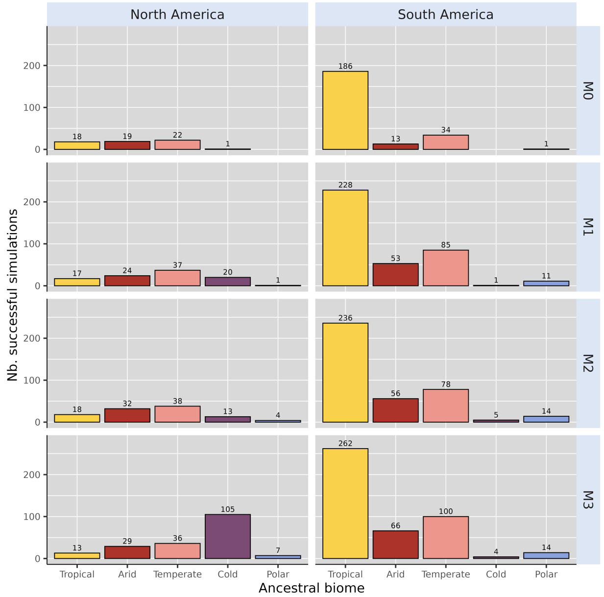
Figure S 8: Biome where the ancestral species of each simulation leading to a successful exchange originated, for each continent and each scenario.
