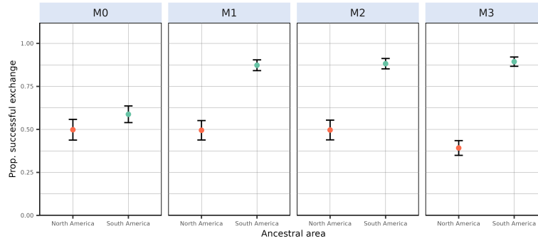
Figure S 2: Proportion of simulations leading to a successful exchange to the other continent after standardising initial distances to the isthmus between both continents (see Section 1). From left to right are depicted the outcome of the zero-adaptationist model ( M0 , species climatic niche does not change through time – climate specialists), full adaptationist model ( M1 , species climatic niche evolves following local environmental conditions – climate generalists) and alternative versions of M1 where species ecological niche is only determined by precipitation ( M2 ) or temperature ( M3 ). Each individual plot shows the outcome of simulations starting in North (red) and South (cyan) America. Dots represent mean proportion estimates computed out of the successful simulations ( i.e. , leading to a successful transcontinental faunal exchange) and error bars show their associated 95% confidence interval derived from a binomial.
