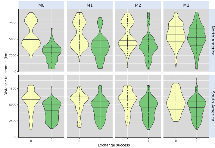
Figure S 5: Comparison of the initial distance to the isthmus between successful and unsuccessful simulations of each of our four models, either starting from North (top) or South (bottom) America. Successful simulations ( Exchange Success = 1) are displayed in green, whereas unsuccessful simulations ( Exchange Success = 0) are displayed in yellow. Dashed lines on top and bottom of the distribution represent the 25% and 75% quantiles whereas the thicker full line in the middle shows the median (50% quantile).
