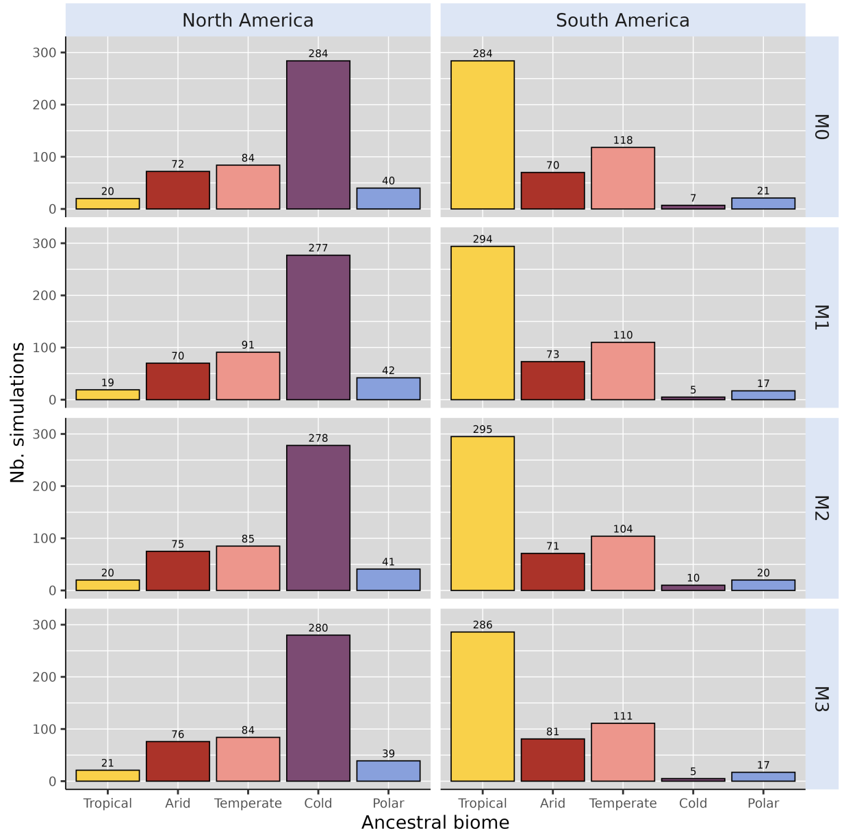
Figure S 7: Biome where the ancestral species of each of the 500 simulation originated, for each continent and each scenario.
