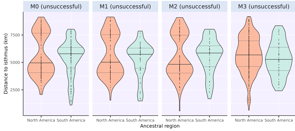
Figure S 4: Distance to the isthmus for non-successful simulations – i.e. , that did not result in a significant interchange. Dashed lines on top and bottom of the distribution represent the 25% and 75% quantiles whereas the thicker full line in the middle shows the median (50% quantile).
