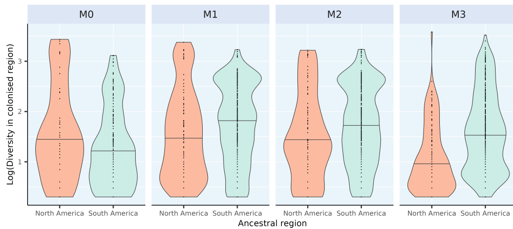
Supp.Figure 2: Diversity in the colonised area following a successful interchange (decimal log scale).
