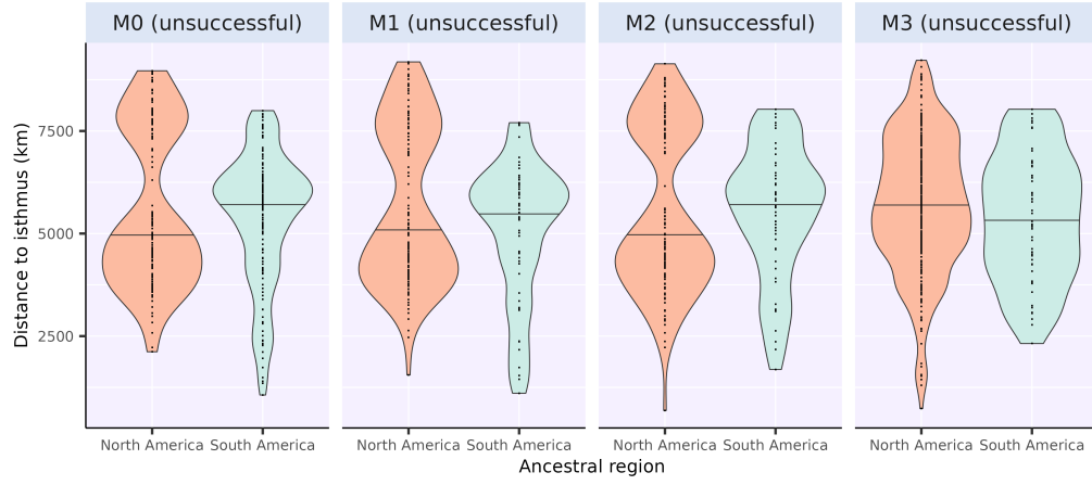
Supp. Figure 3: Distance to the isthmus for non-successful simulations – i.e. , that did not result in a significant interchange.
