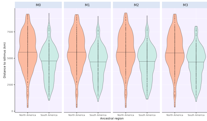
Supp.Figure 1: Distribution of the distance to isthmus of the ancestral species of simulations either starting in North or South America, resulting from our random equal-area sampling scheme (see Method details)
