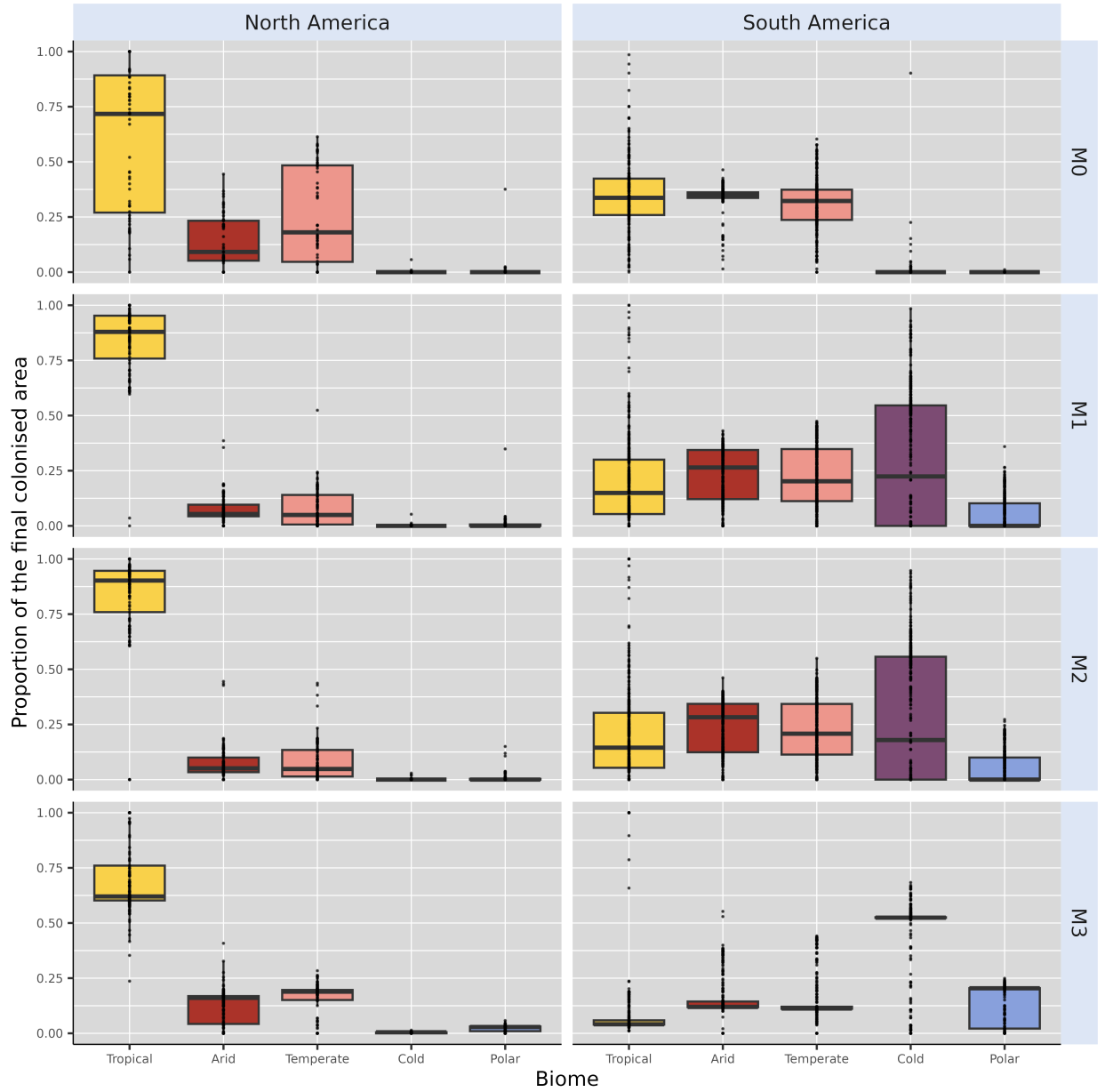
Figure 3: Proportion of the final area occupied within each biome after each successful simulation. Rows discriminate the model that generated simulations (from M0 to M3 ), and columns the continent where the simulation started (either North or South America).
