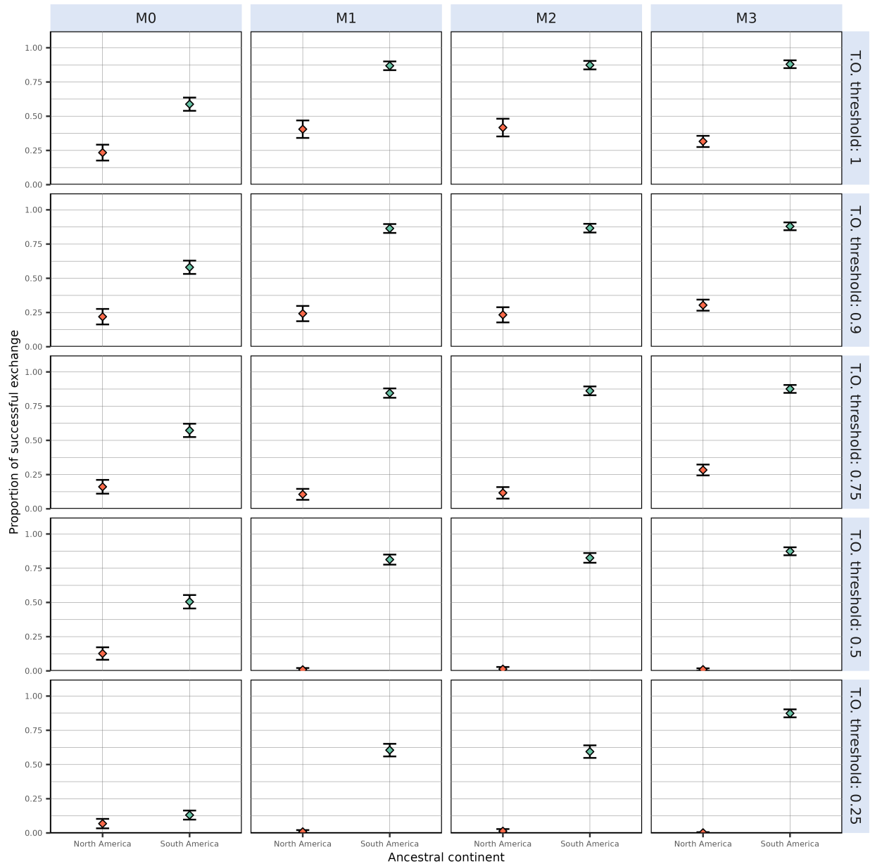
Figure 2: Proportion of successful exchanges after removing runs with different levels of tropical occupancy (T.O.) within the colonised continent, for each initial landmass-modelling scenario combination. For each successful run, T.O. was quantified as the proportion of colonised area assigned to the tropical biome. Success proportions were further assessed after removing runs with proportion of colonised area above a given threshold of T.O., ranging from 25% to 100% of the colonised area.
