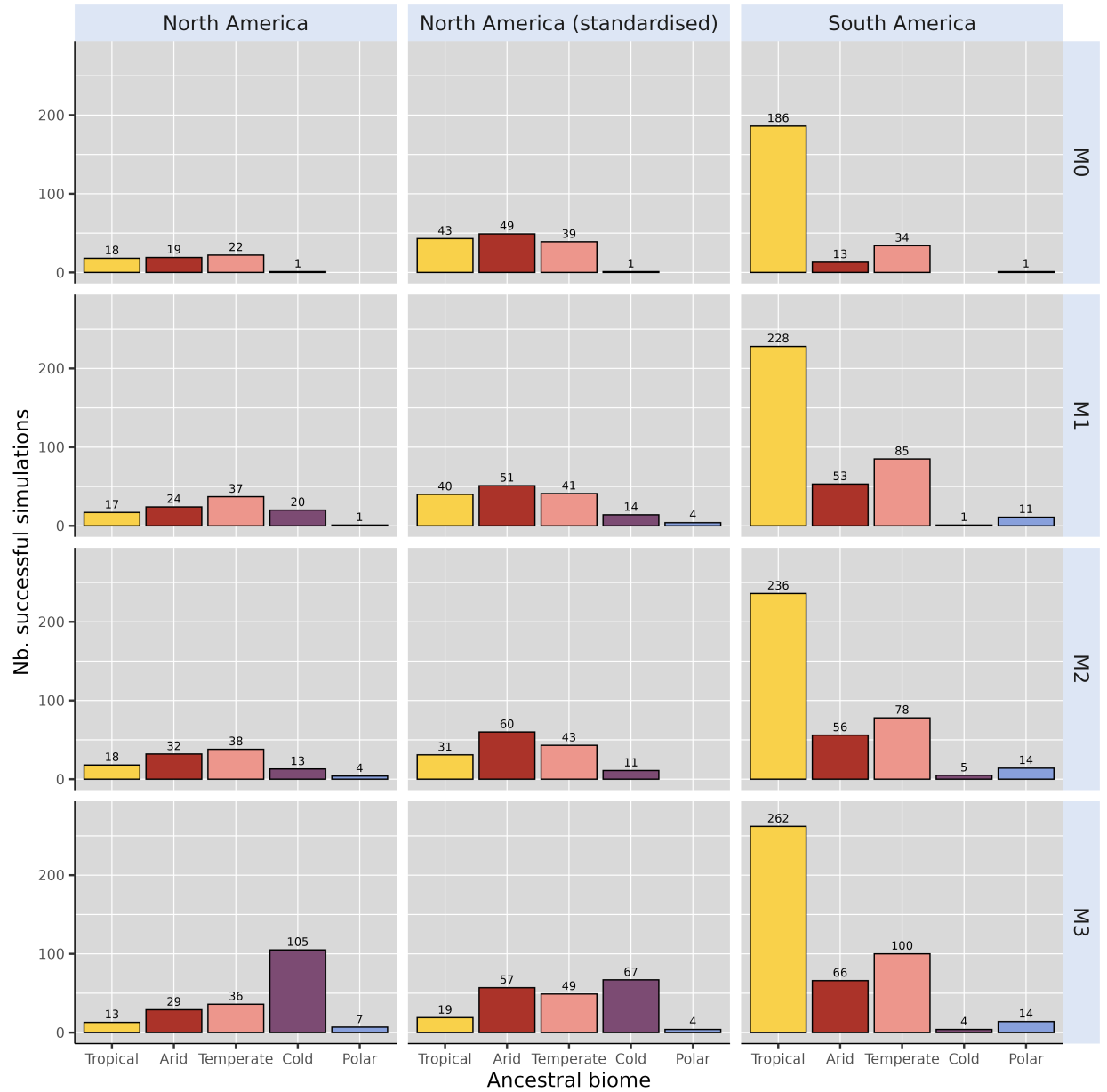
Figure 1: Biome where the ancestral species of each simulation leading to a successful exchange originated, for each continent and each scenario. “North America standardised” refers to simulations starting from North America after standardising initial distance to isthmus with that of simulations starting from South America (see Material and Methods and Figure S2).
