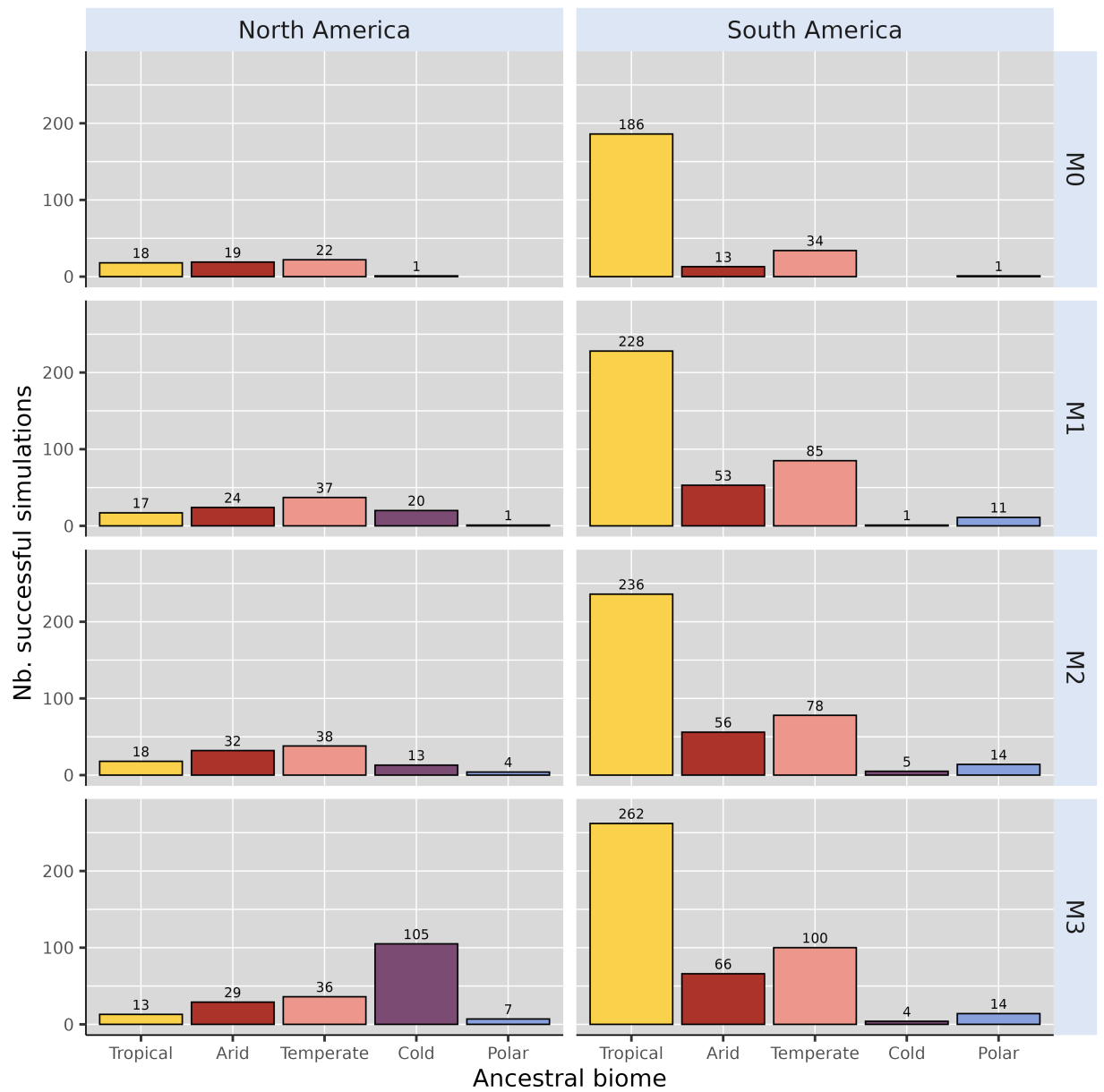
Figure S 10: Biome where the ancestral species of each simulation leading to a successful exchange originated, for each continent and each scenario.
