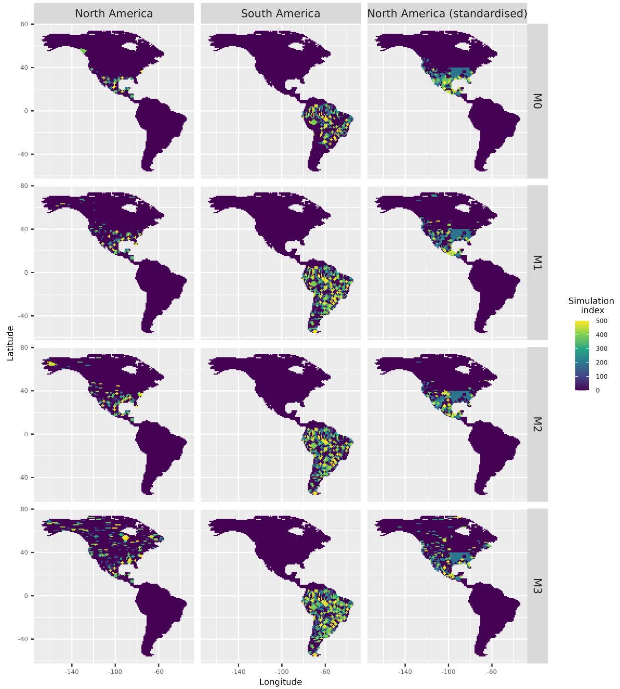
Figure S 3: Starting range of successful simulations generated under each model (from M_0 to M_3 ), either starting from North America ( left ), South America ( middle ) or North America after standardising initial distances to the isthmus with those from South America ( right ).
