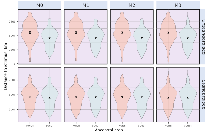
Figure S 1: Initial distances to the isthmus of all simulations ( n = 500 ), either starting from North or South America. On the top row, locations of simulation's ancestral species resulted from a random landmass-scale equal-area sampling scheme, both starting from North and South America. On the bottom row, initial distances to the isthmus of simulations originating in North America were standardised to those of South America (see Section 1). Note that no change was made for simulations starting from South America.
