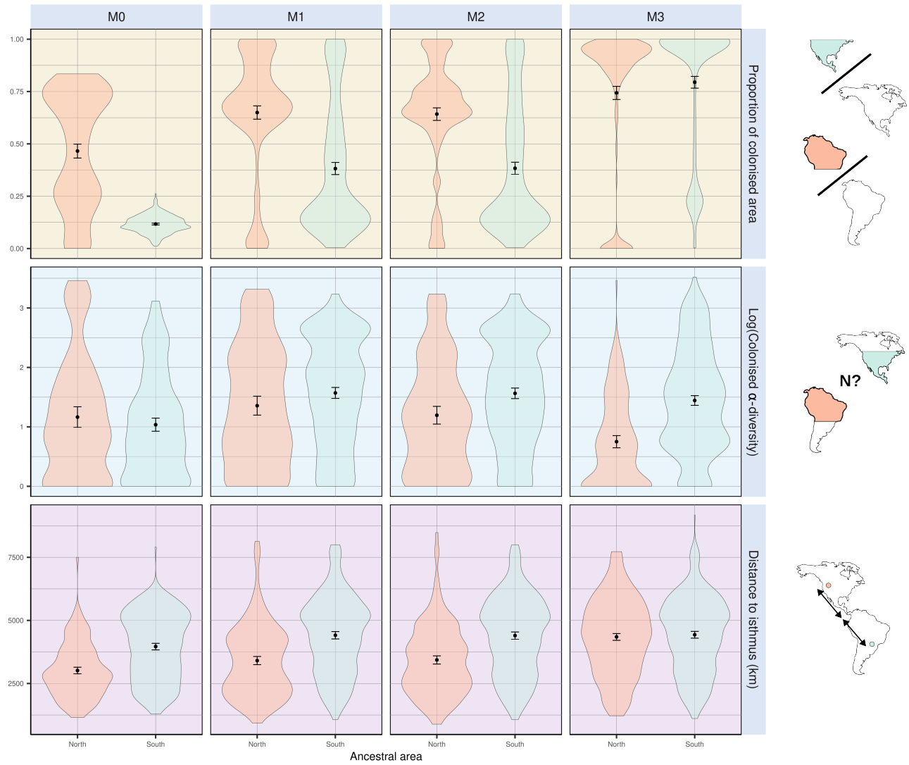
Figure S 5: A few metrics summarising climate-mediated interchange after standardising initial distances to the isthmus of simulations starting from North America to those starting from South America. Each individual plot shows the outcome of simulations starting in North (red) and South (cyan) America. ( top ) Proportion of foreign continent's colonised area. ( middle ) Diversity within the colonised area. ( bottom ) Distance to the isthmus. The first two metrics have been computed out of successful simulations, i.e. , that resulted in a transcontinental faunal exchange.
