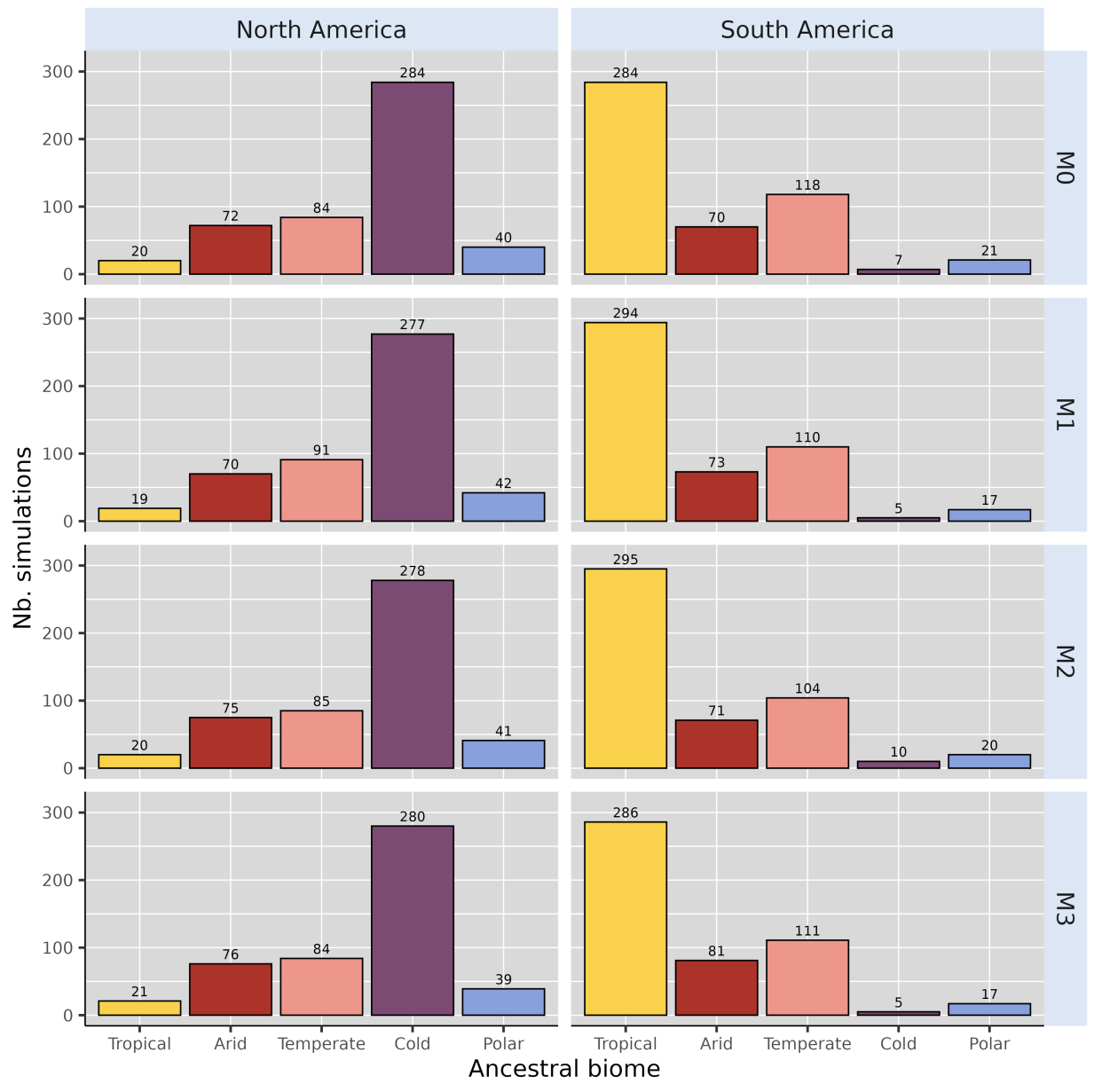
Figure S 9: Biome where the ancestral species of each of the 500 simulation originated, for each continent and each scenario.
