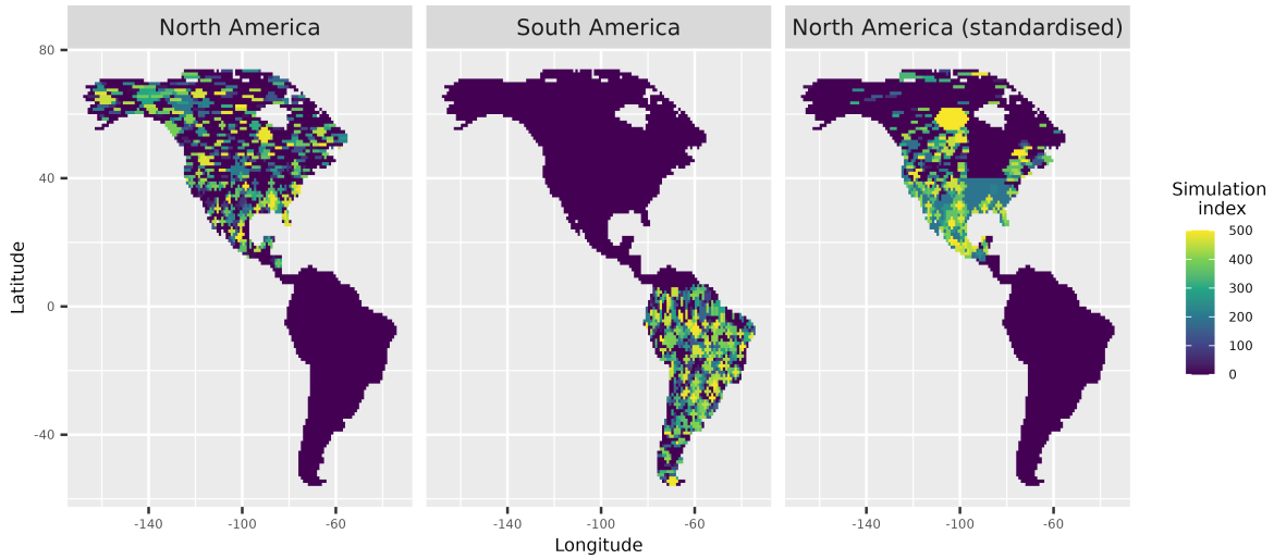
Figure S 2: Starting range of all simulations either starting from North America ( left ), South America ( middle ) or North America after standardising initial distances to the isthmus with those from South America ( right ).
