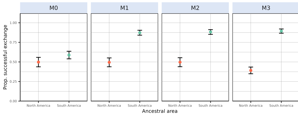
Figure S 4: Proportion of simulations leading to a successful exchange to the other continent after standardising initial distances to the isthmus between both continents (see Section 1). From left to right are depicted the outcome of the zero-adaptationist model ( M0 , species climatic niche does not change through time – climate specialists), full adaptationist model ( M1 , species climatic niche evolves following local environmental conditions – climate generalists) and alternative versions of M1 where species ecological niche is only determined by precipitation ( M2 ) or temperature ( M3 ). Each individual plot shows the outcome of simulations starting in North (red) and South (cyan) America. Dots represent mean proportion estimates computed out of the successful simulations ( i.e. , leading to a successful transcontinental faunal exchange) and error bars show their associated 95% confidence interval derived from a binomial.
