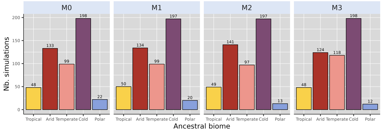
Figure S 9: Biome where the ancestral species of each of the 500 simulation originated, for each modelling scenario, starting from North America after standardising initial distance to isthmus with that of simulations starting from South America (see Section 1.2 and Figure S1). We removed simulations starting from a cell that could not be assigned a biome from our counts, hence the reason why some are not exactly summing to 500.
