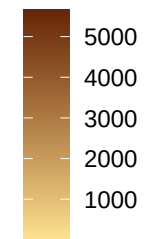
Elevation (m)
