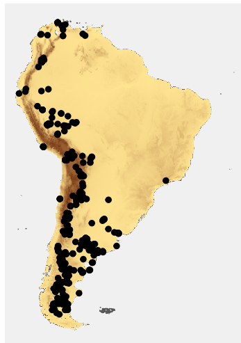
Miocene
