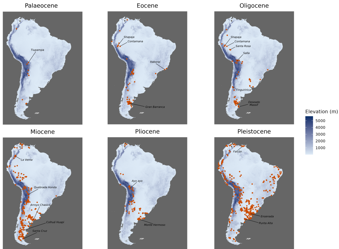
Figure 4.1: Distribution of the South American mammal fossil record across geological epochs (Holocene excluded), on top of the continent's present-day topography ( Boschman 2021 ). Several keystone localities have been highlighted.
