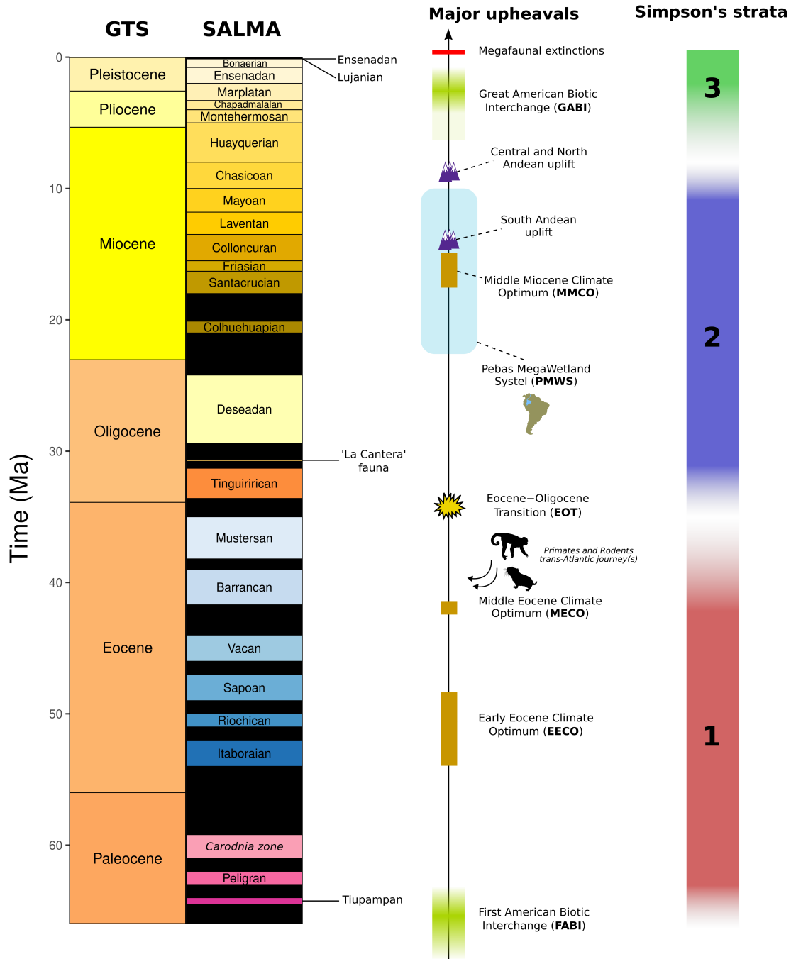
Figure 4.2: Integrative view of the Cenozoic of South America from the land mammal perspective. The South American Land Mammal Age (SALMA) scale used all over this thesis is shown, along with the corresponding Geological Time Scale (GTS) epochs, from the International Chronostratigraphic Chart (v2024/12) (Holocene not depicted). Boundaries between SALMAs were defined on the basis of the most up-to-date literature ( e.g. , Bellinzoni et al. 2025 ; Dunn et al. 2013 ; Gelfo et al. 2009 ; Woodburne et al. 2014 ), but note that many intervals lack absolute temporal calibration. Black spaces between SALMAs represent temporal gaps. Alongside are depicted several key biotic or abiotic upheaval in the Cenozoic history of South American mammals, as well as Simpson's three faunal strata ( Simpson 1980 ). Silhouettes are from Phylopic (credit: Sarah Werning and Kai R. Caspar).
