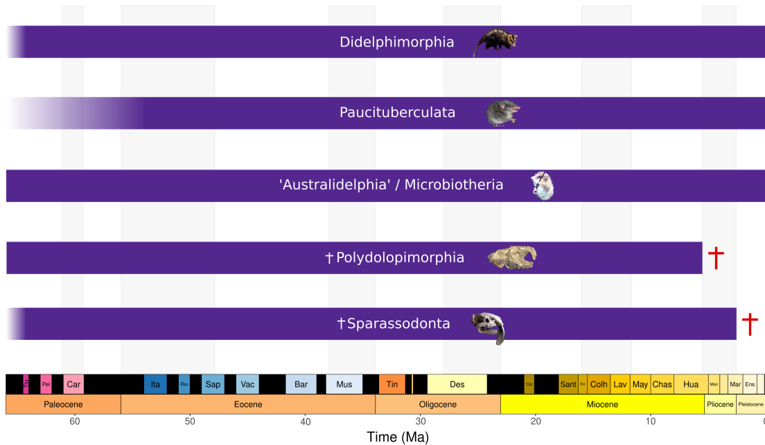
Figure 4.4: Order-level persistence of South American metatherians in the fossil record. Fading colours mean that the group has no known fossil record for the period, but should already exist. Photos were taken from iNaturalist (credit: Jorge Brito, Eduardo Silva Rodriguez, Thiago Chagas). Wamradolops telloi cranium comes from Stutz et al. (2026), reproduced with permission. The picture of the Thylacosmilus atrox cranium was taken by Claire Houck
