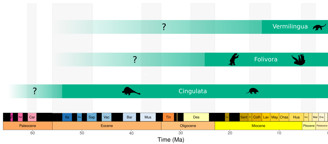
Figure 4.6: Higher-level persistence of xenarthrans in the fossil record. Fading colours with question marks depict the ‘xenarthran mystery’, i.e. , that the group in question has no known fossil record for the period, but should already exist. Divergence ages between the main lineages were taken from Tejada et al. (2024). Vermilingua and Folivora altogether form the order Pilosa. Silhouettes are from Phylopic (credit: Julián Bayona and Sarah Werning).
