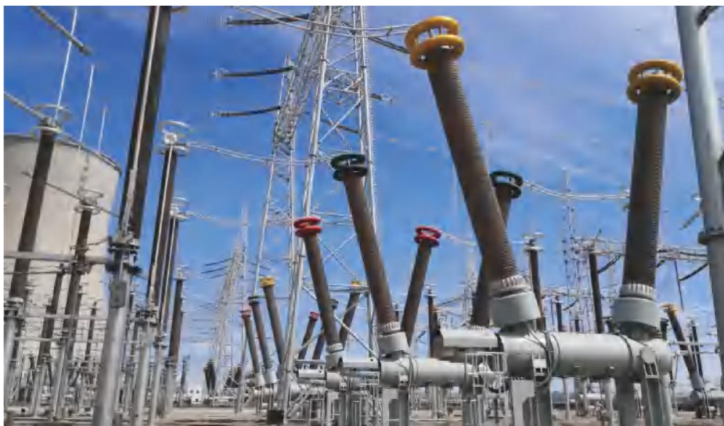
800kV SF6 tank-type circuit breaker
