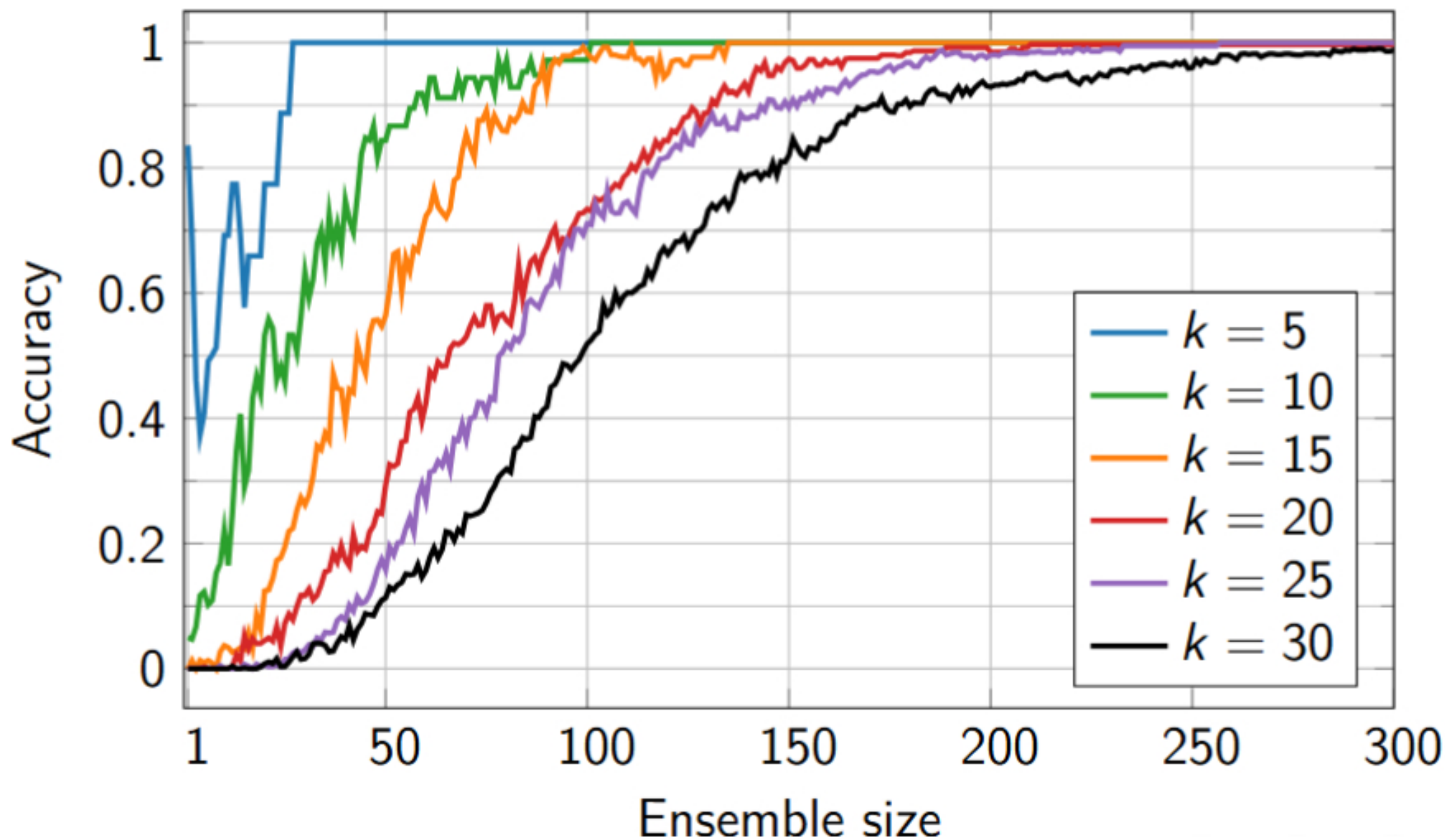
Experiment 2 Accuracy vs ensemble size
