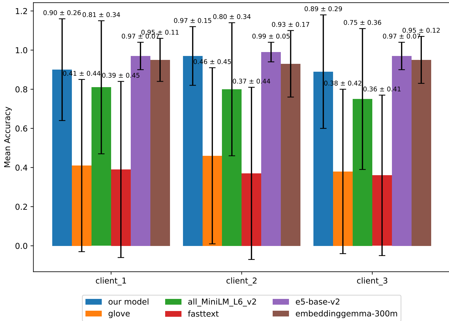
Our Best Model vs. Pretrained Models
