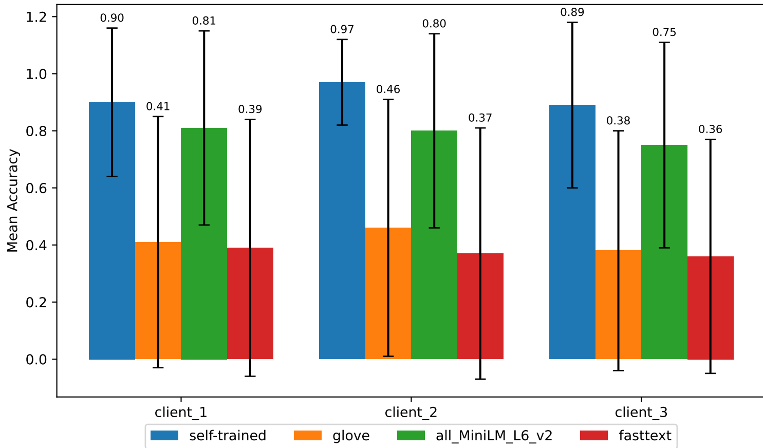
Best Self-Trained vs. Pretrained Models
