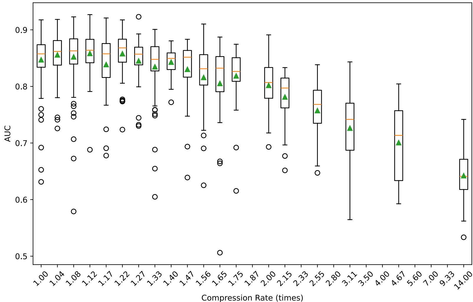
AUC vs Compression Rate
