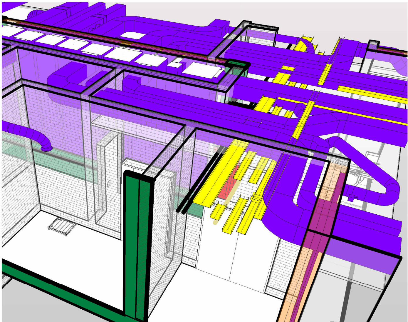
Ward Passage Ceiling Void _Coordination
