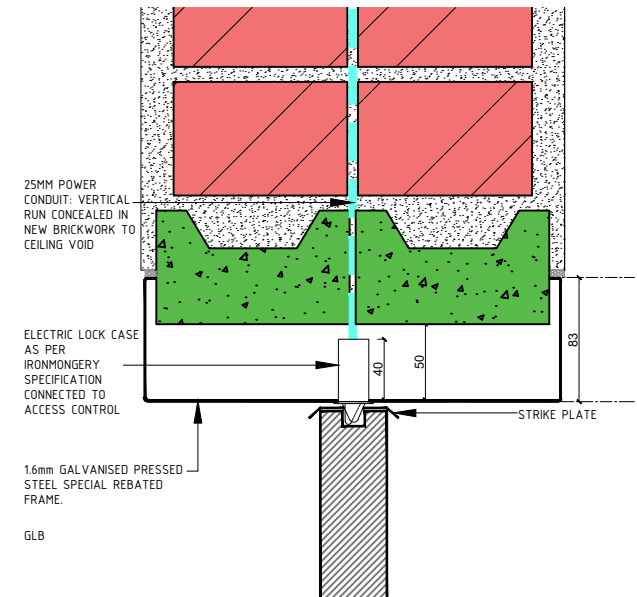
SECTION SCALE 1:5
