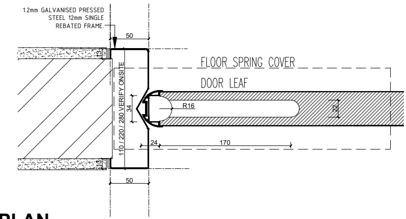
PLAN SCALE 1:5
