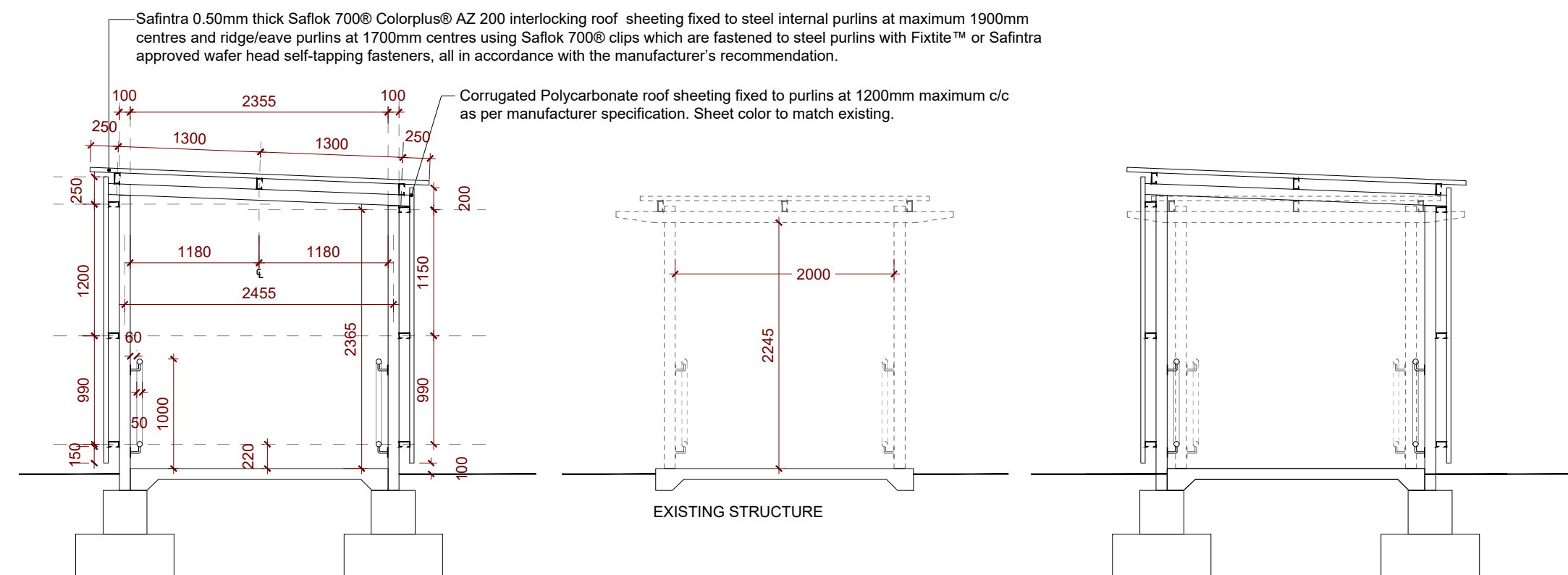
BUILDING SECTION 01 SCALE 1:50
