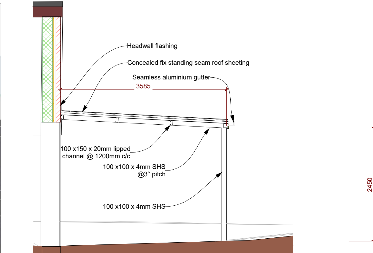
BUILDING SECTION 02 SCALE 1:50
