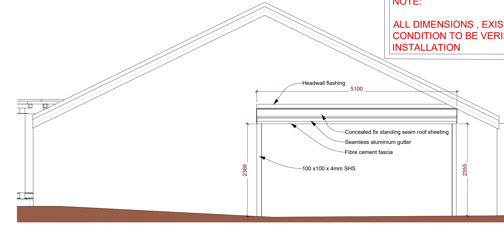
BUILDING ELEVATION SCALE 1:50
