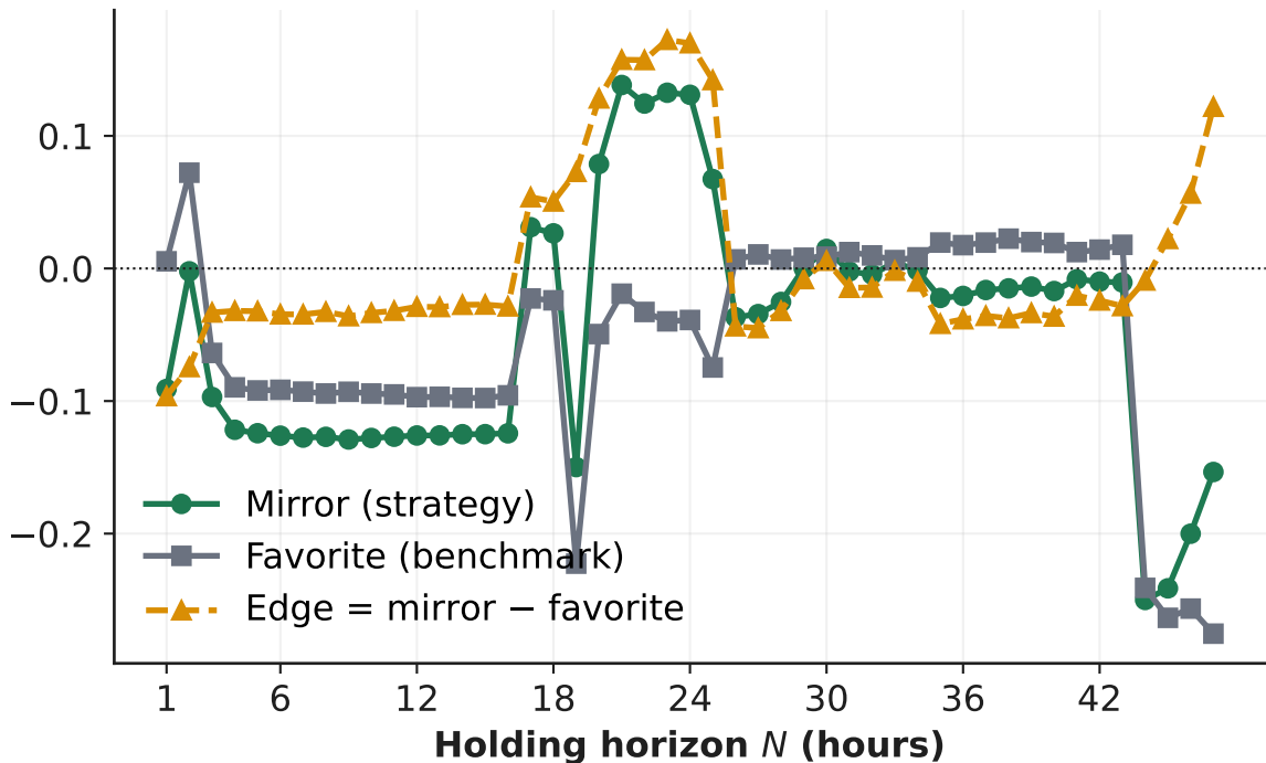
Gross return
