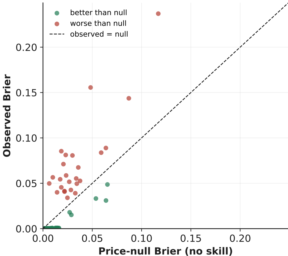
Study 1: no wallet beats its price-null significantly
