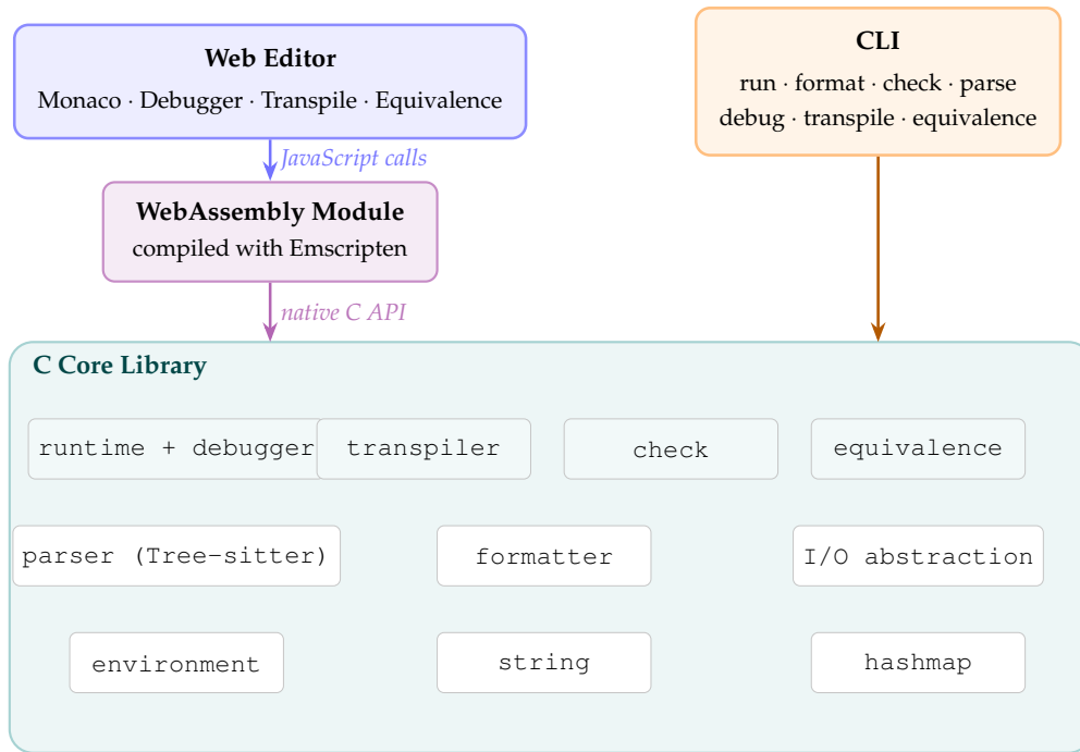
Figure 4.1: Compile-time dependency graph of the Pseudo++ modules, grouped by layer. The C core library (teal) is compiled to both a native CLI binary and a WebAssembly module loaded by the web editor.
