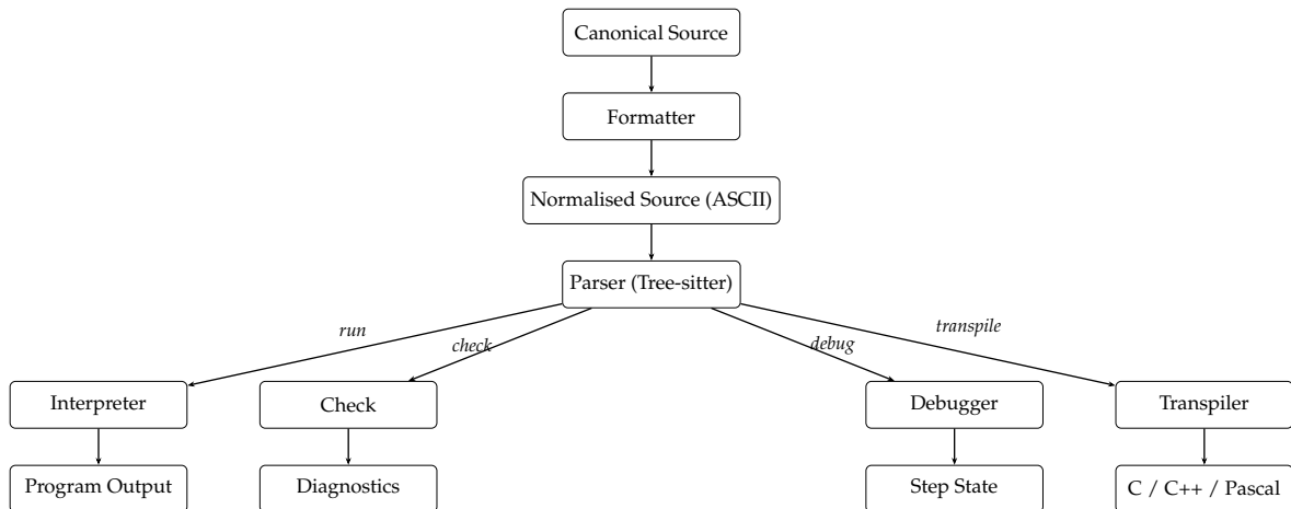
Figure 3.1: The Pseudo++ processing pipeline. After normalisation and parsing, the CST is handed to the interpreter, static analyser, debugger, or transpiler depending on the requested operation.
