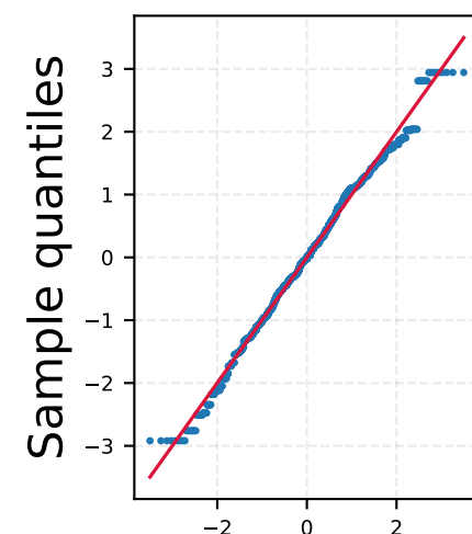
Theoretical quantil
