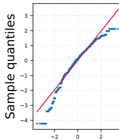
Theoretical quantiles
