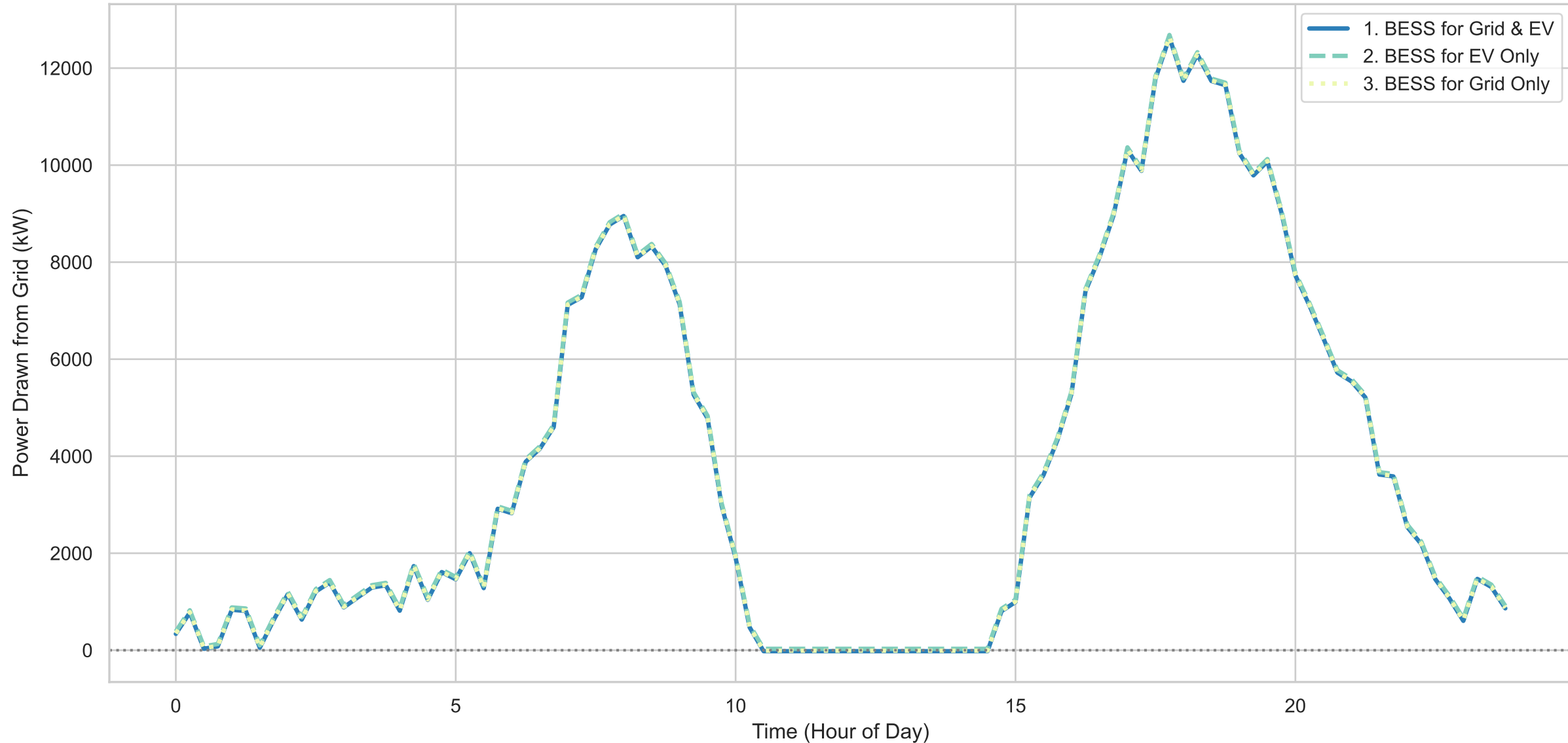
Case 3: Grid Peak Shaving Comparison
