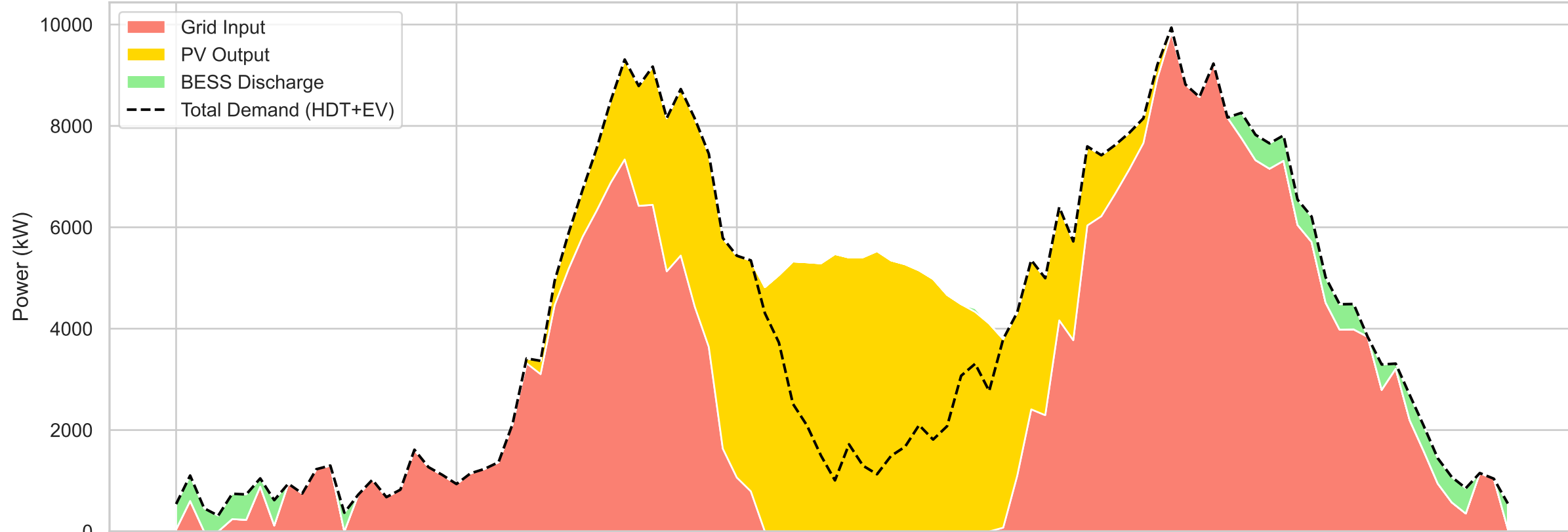
Energy Flow: Scheduled Fleet
