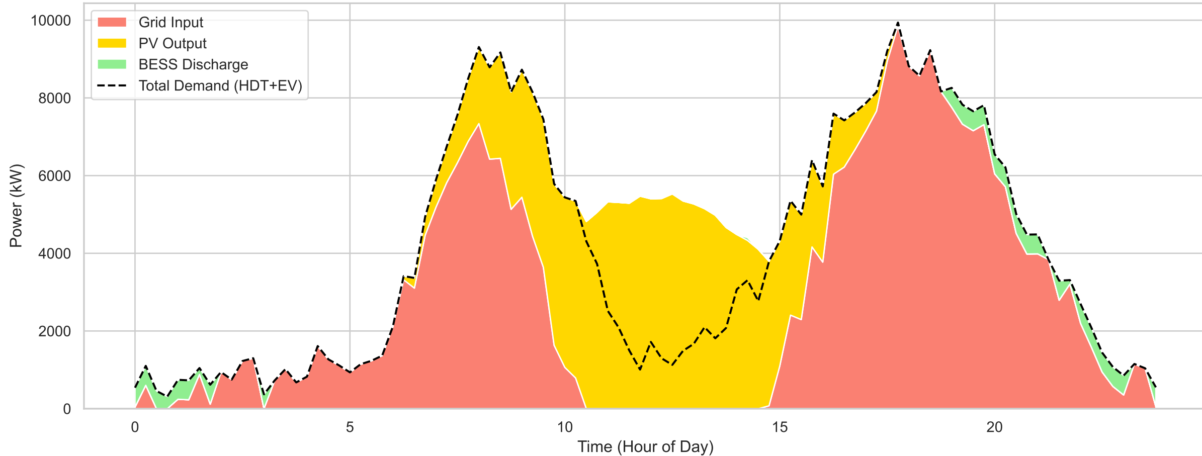
Energy Flow: Unscheduled Fleet
