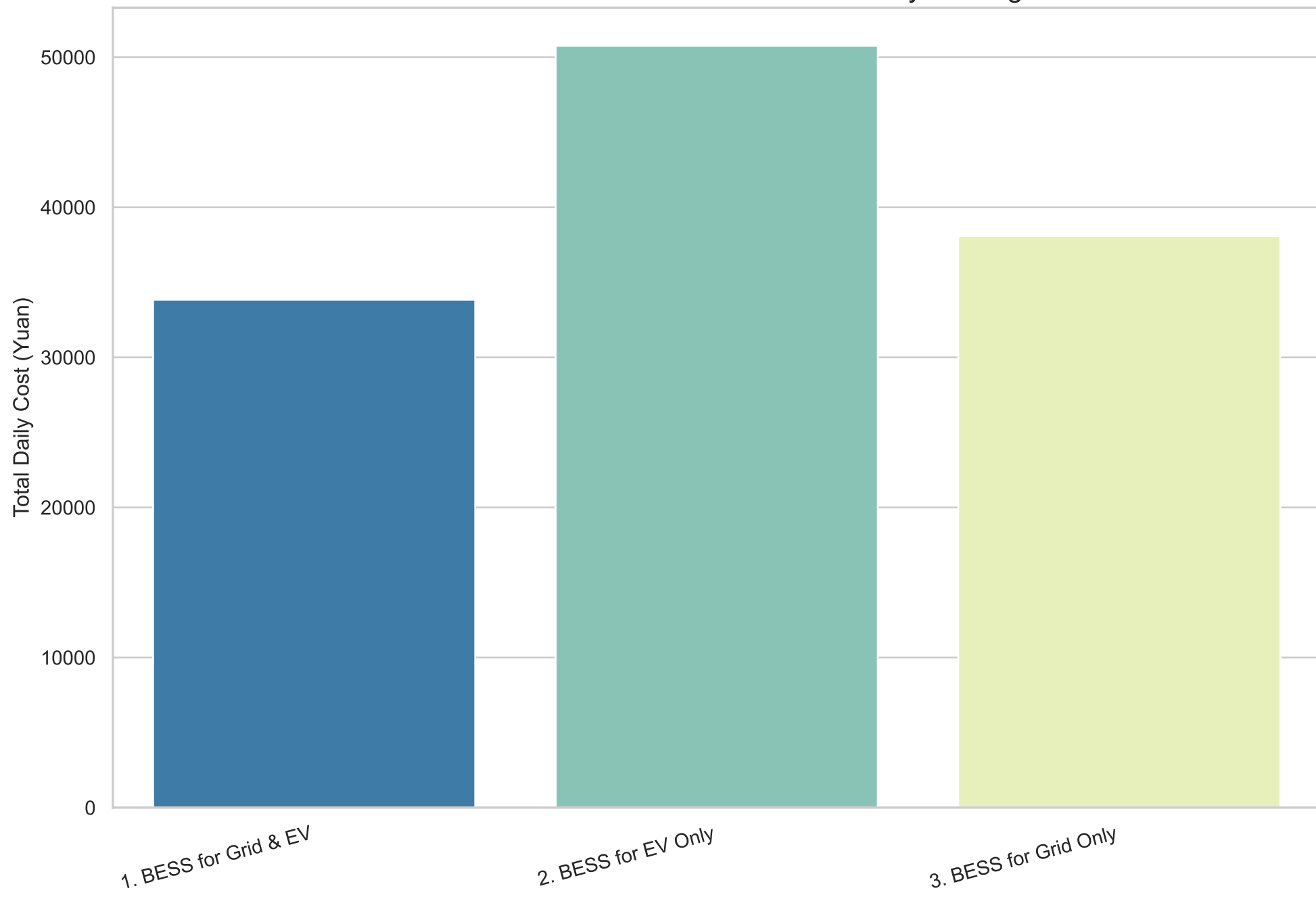
Case 3: Economic Cost of Different Battery Strategies
