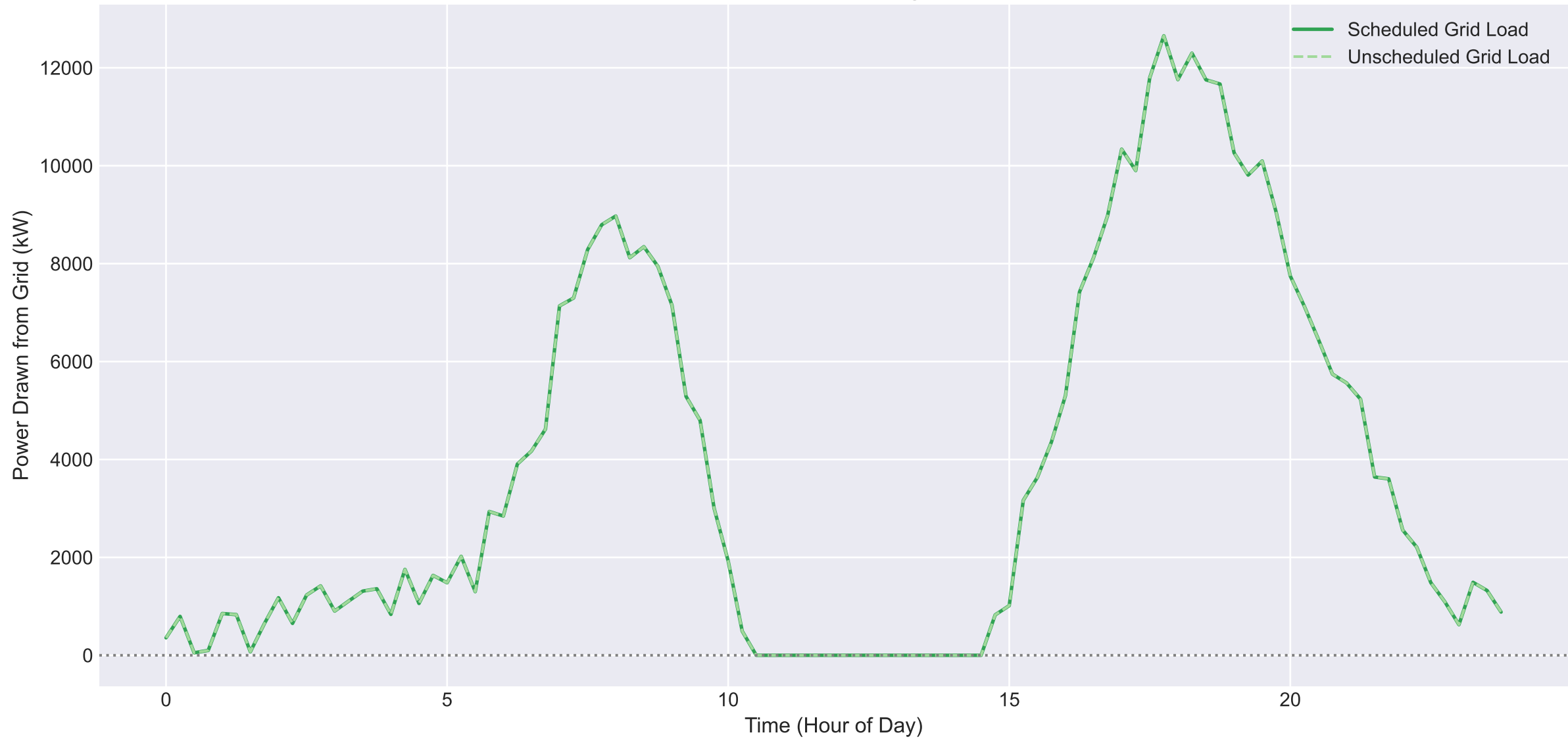
Case 1: Grid Peak Shaving Comparison
